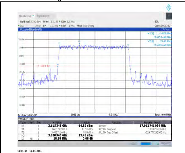
1-N48-30-20-M-1-DFT-QPSK-Outer_Full-50@0-Ant0 -17.913-18.880-≤20-PASS
