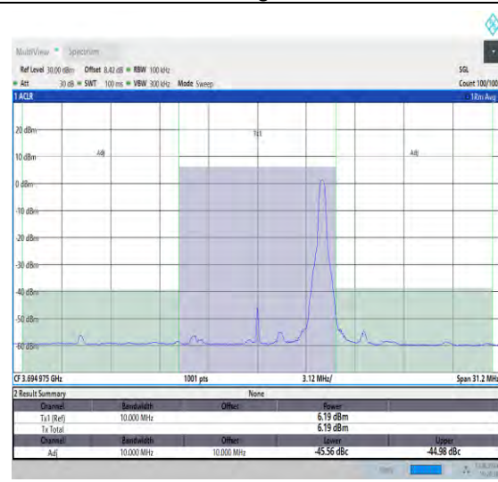
NTNV_N48_PC3_30_10_H_TID6_#1_-10_10
