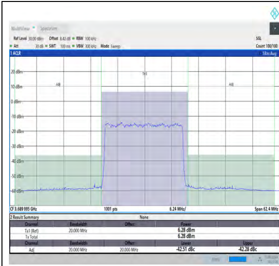
NTNV_N48_PC3_30_20_H_TID1_#1_-20_20
