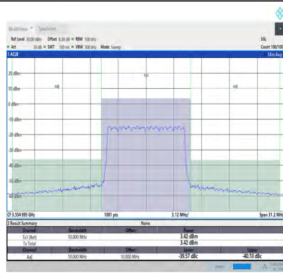
NTNV_N48_PC3_30_10_L_TID19_#1_-10_10
