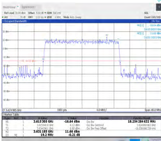
1-N48-30-20-M-6-CP-QPSK-Outer_Full-51@0-Ant0 18.254-19.200-≤20-PASS
