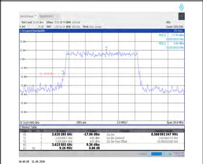
1-N48-30-10-M-8-CP-64QAM-Outer_Full-24@0-Ant 0-8.568-9.260≤10-PASS
