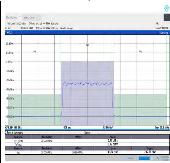
NTNV_N48_PC3_30_30_H_TID25_#1_-30_30
