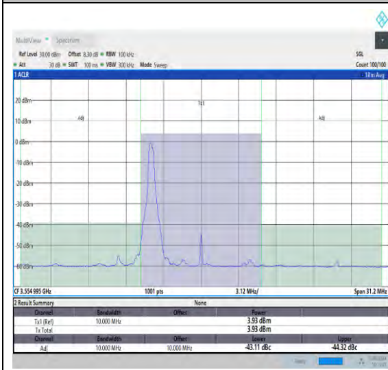
NTNV_N48_PC3_30_10_L_TID11_#1_-10_10
