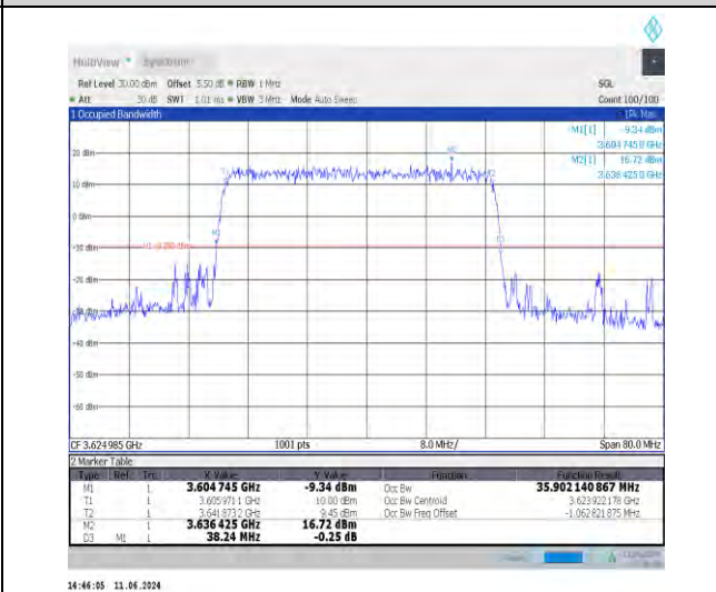
1-N48-30-40-M-1-DFT-QPSK-Outer_Full-100@0-Ant0 0-35.902-38.240-≤40-PASS
