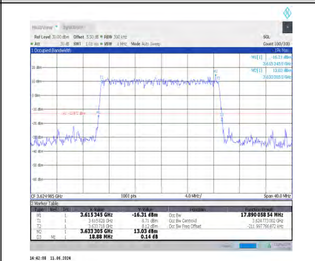
1-N48-30-20-M-3-DFT-16QAM-Outer_Full-50@0-Ant 0-17.89-18.880-≤20-PASS
