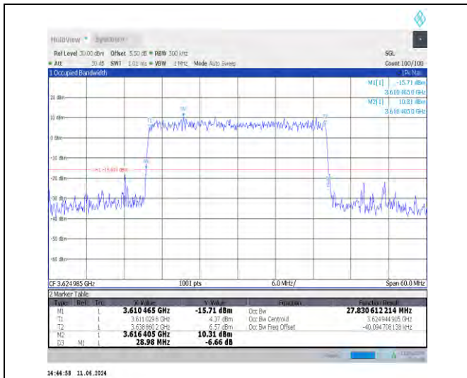
1-N48-30-30-M-7-CP-16QAM-Outer_Full-78@0-Ant0 -27.831-28.980-≤30-PASS
