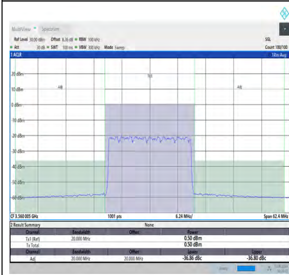
NTNV_N48_PC3_30_20_L_TID25_#1_-20_20
