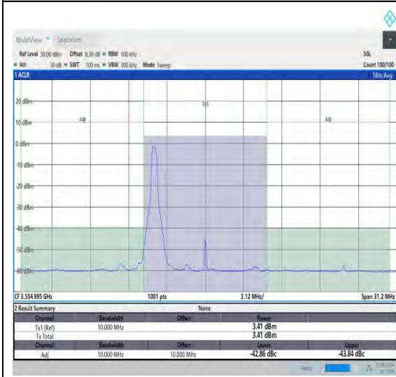
NTNV_N48_PC3_30_10_L_TID17_#1_-10_10
