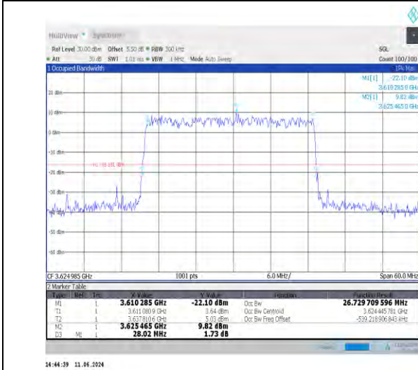
1-N48-30-30-M-5-DFT-256QAM-Outer_Full-75@0-A nt0-26.732-28.020-≤30-PASS
