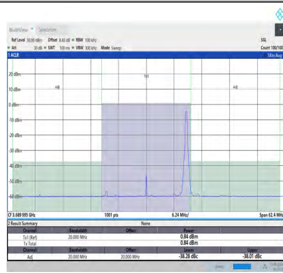
NTNV_N48_PC3_30_20_H_TID27_#1_-20_20
