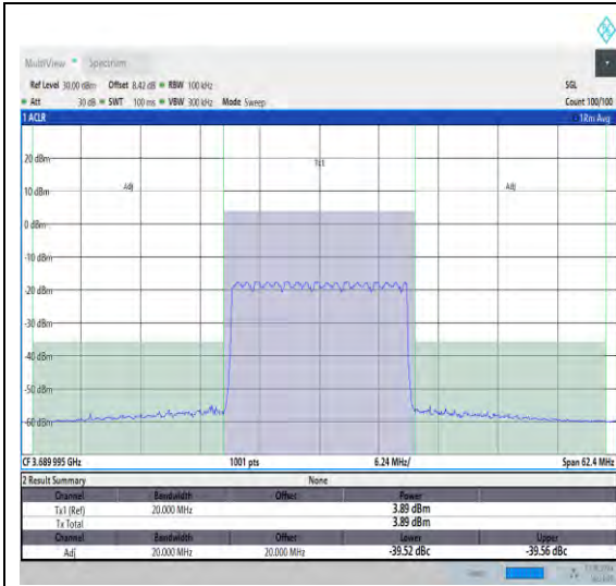
NTNV_N48_PC3_30_20_H_TID16_#1_-20_20
