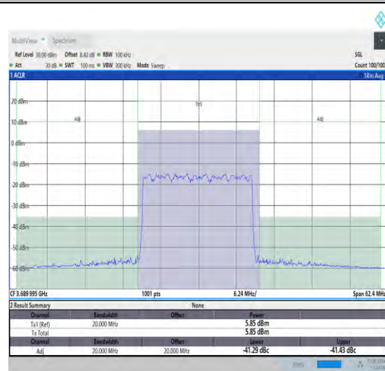
NTNV_N48_PC3_30_20_H_TID4_#1_+20_20
