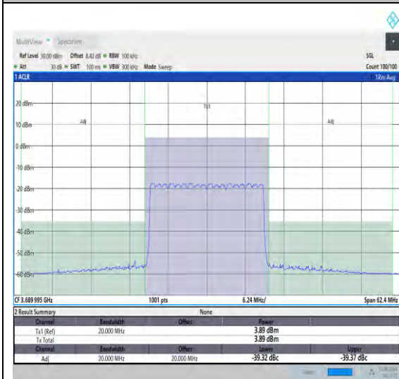
NTNV_N48_PC3_30_20_H_TID19_#1_-20_20
