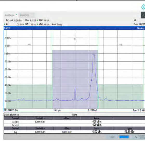
NTNV_N48_PC3_30_10_H_TID18_#1_-10_10
