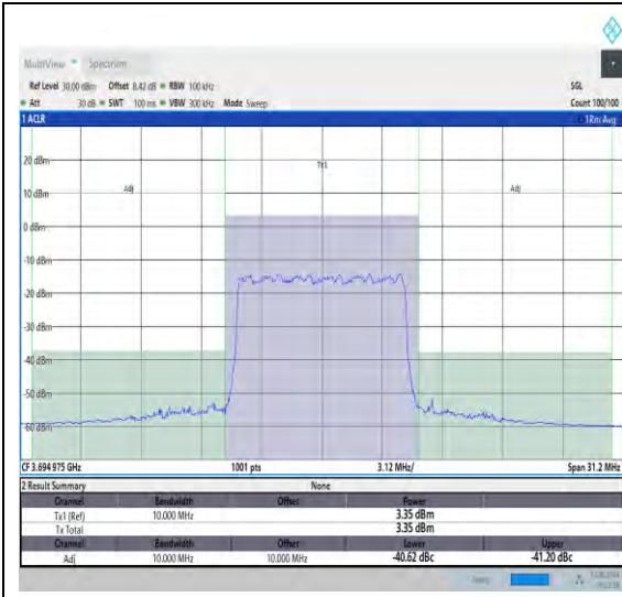
NTNV_N48_PC3_30_10_H_TID22_#1_-10_10
