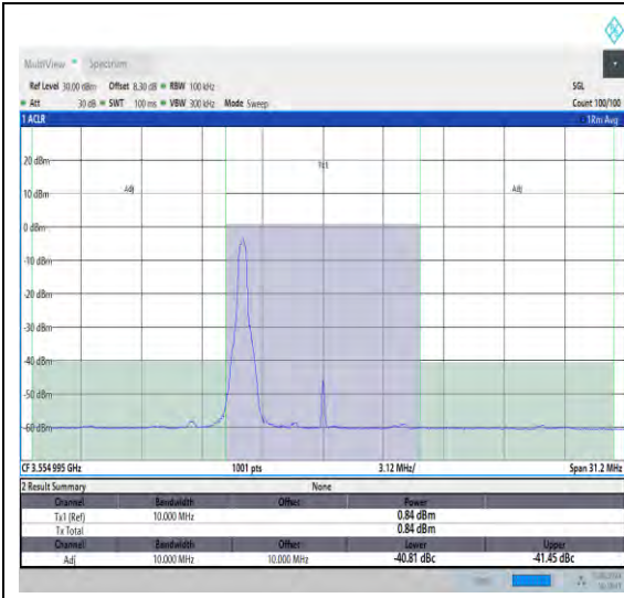
NTNV_N48_PC3_30_10_L_TID26_#1_-10_10
