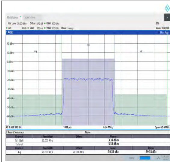
NTNV_N48_PC3_30_20_H_TID22_#1_-20_20
