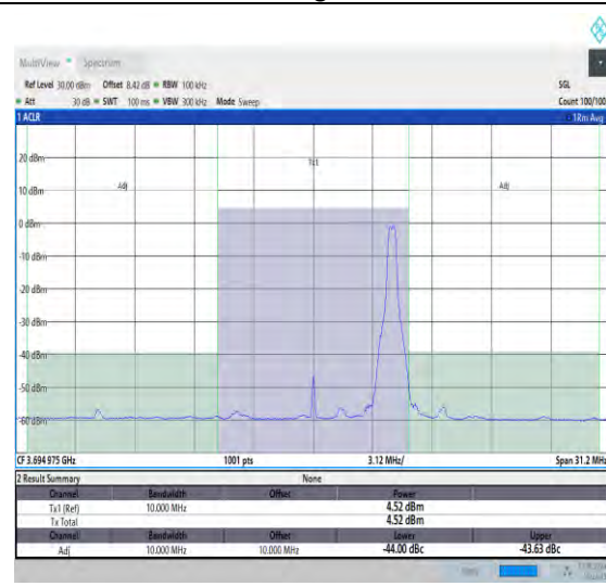
NTNV_N48_PC3_30_10_H_TID12_#1_-10_10
