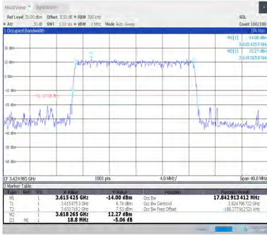
1-N48-30-20-M-4-DFT-64QAM-Outer_Full-50@0-Ant 0-17.843-18.800-≤20-PASS
