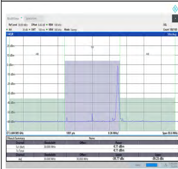
NTNV_N48_PC3_30_30_H_TID21_#1_-30_30
