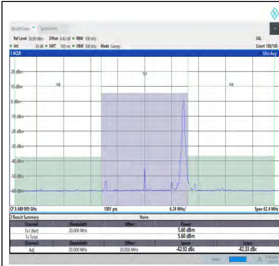
NTNV_N48_PC3_30_20_H_TID6 #1_-20_20
