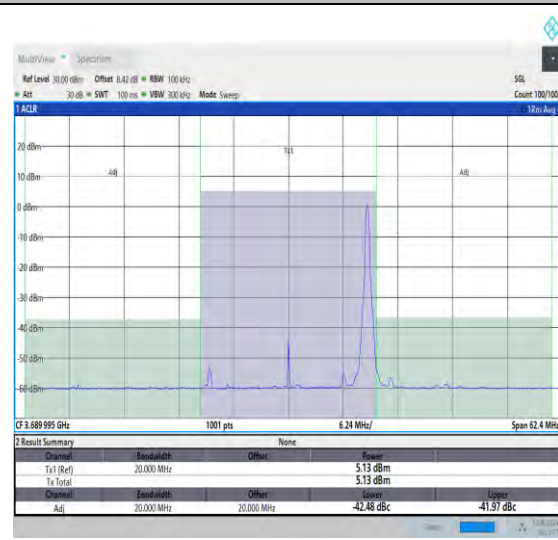
NTNV_N48_PC3_30_20_H_TID9 #1_-20_20
