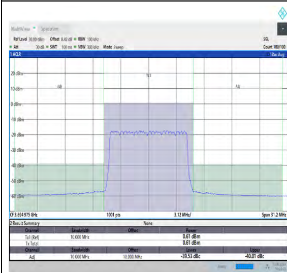
NTNV_N48_PC3_30_10_H_TID25_#1_-10_10
