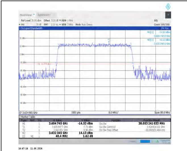
1-N48-30-40-M-6-CP-QPSK-Outer_Full-106@0-Ant0 -38.053-40.400-≤40-PASS
