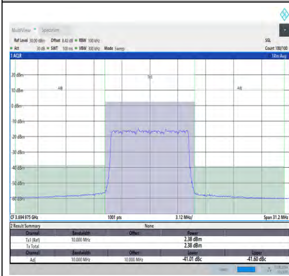
NTNV_N48_PC3_30_10_H_TID13_#1_-10_10
