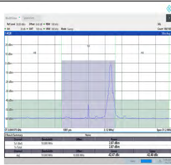
NTNV_N48_PC3_30_10_H_TID15_#1_-10_10
