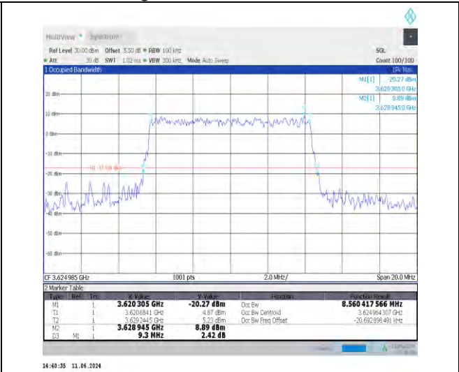
1-N48-30-10-M-6-CP-QPSK-Outer_Full-24@0-Ant0- 8.56-9.300≤10-PASS
