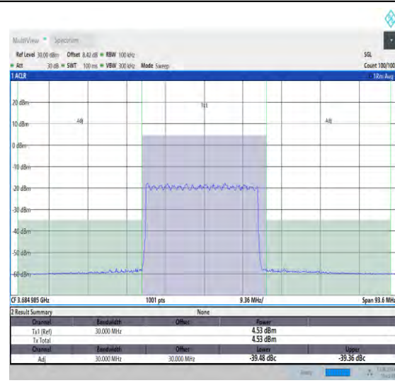
NTNV_N48_PC3_30_30_H_TID10_#1_30_30
