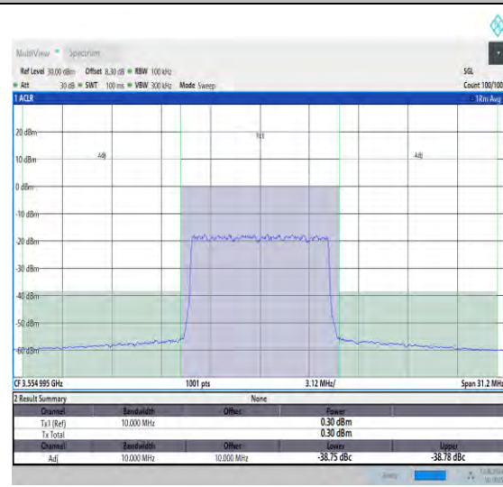
NTNV_N48_PC3_30_10_L_TID25_#1_-10_10
