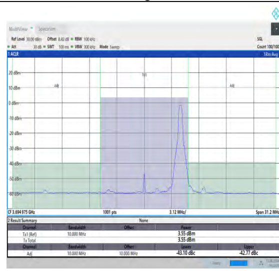
NTNV_N48_PC3_30_10_H_TID24_#1_-10_10
