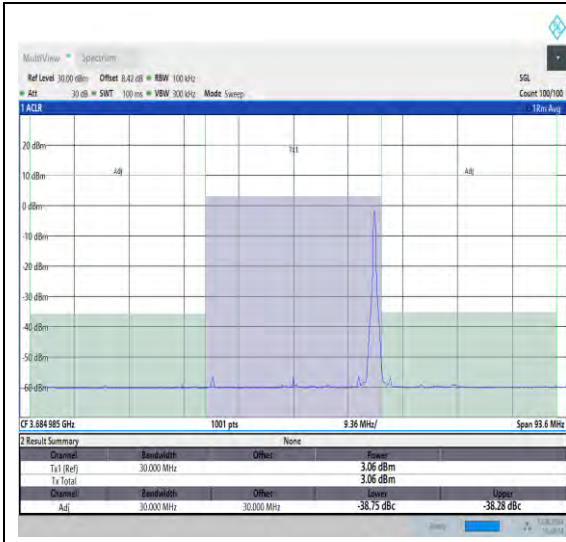
NTNV_N48_PC3_30_30_H_TID24_#1_-30_30
