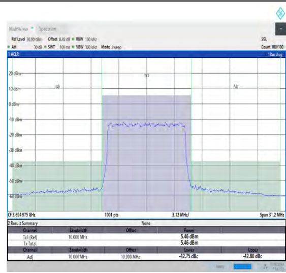
NTNV_N48_PC3_30_10_H_TID4_#1_-10_10
