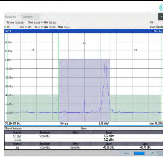
NTNV_N48_PC3_30_10_H_TID27_#1_-10_10
