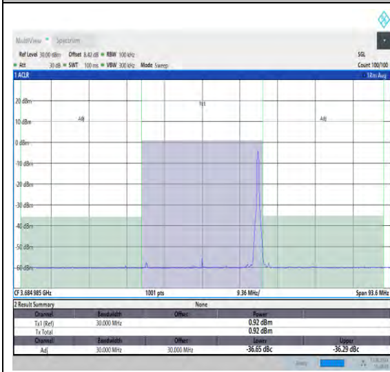
NTNV_N48_PC3_30_30_H_TID27_#1_-30_30
