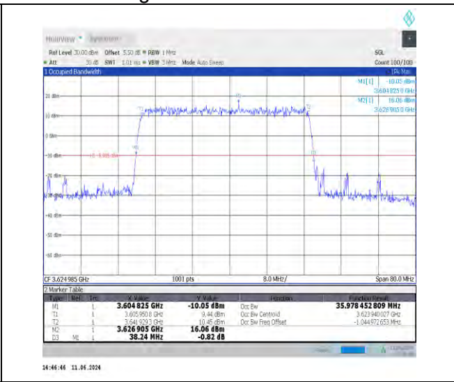
1-N48-30-40-M-3-DFT-16QAM-Outer_Full-100@0-Ant0-35.978-38.240-≤40-PASS
