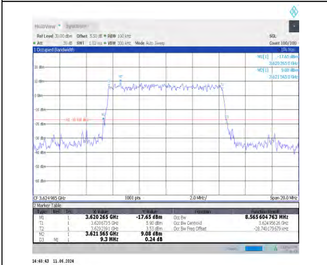
1-N48-30-10-M-7-CP-16QAM-Outer_Full-24@0-Ant0 -8.566-9.300≤10-PASS
