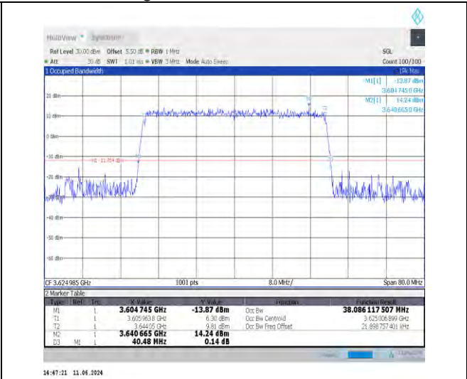
1-N48-30-40-M-7-CP-16QAM-Outer_Full-106@0-Ant0 -38.086-40.480-≤40-PASS
