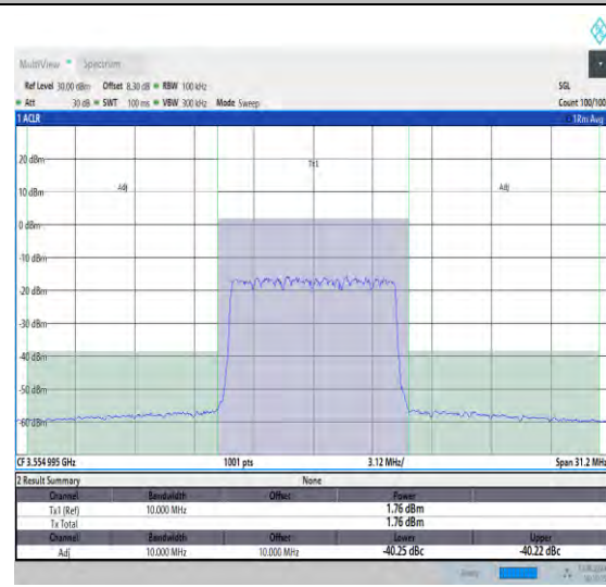
NTNV_N48_PC3_30_10_L_TID13_#1_-10_10
