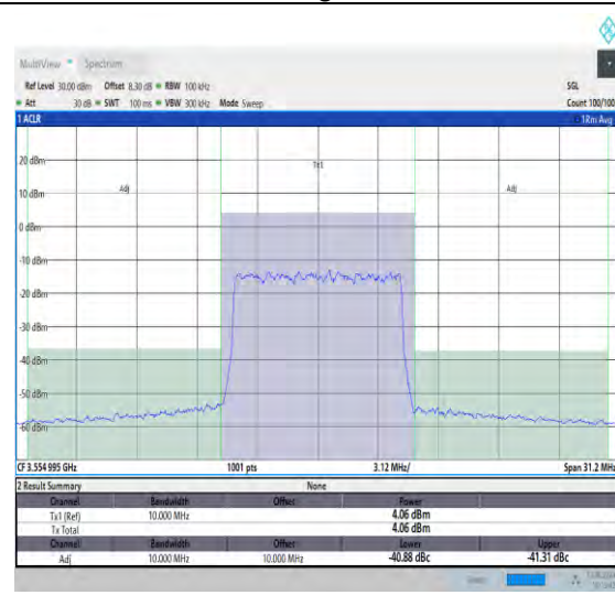
NTNV_N48_PC3_30_10_L_TID10_#1_-10_10
