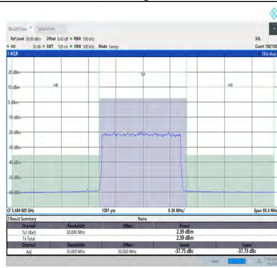
NTNV_N48_PC3_30_30_H_TID13_#1_30_30
