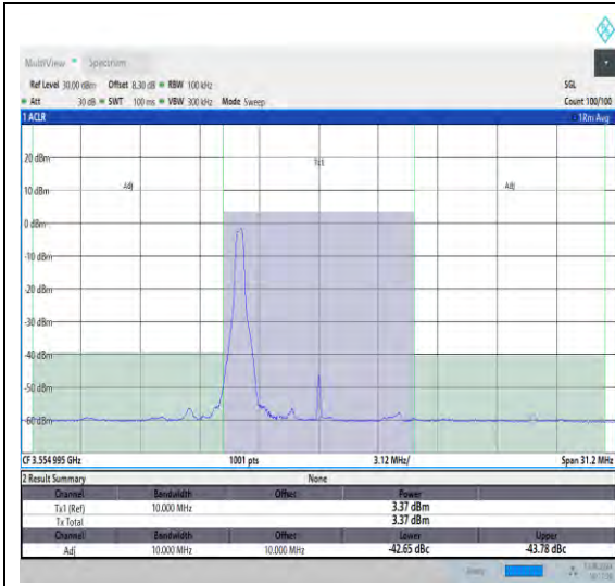
NTNV_N48_PC3_30_10_L_TID20_#1_-10_10
