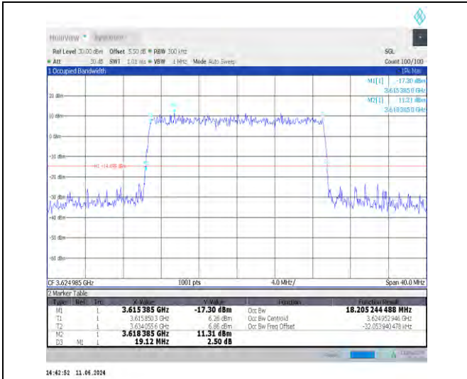
1-N48-30-20-M-8-CP-64QAM-Outer_Full-51@0-Ant0 -18.205-19.120-≤20-PASS
