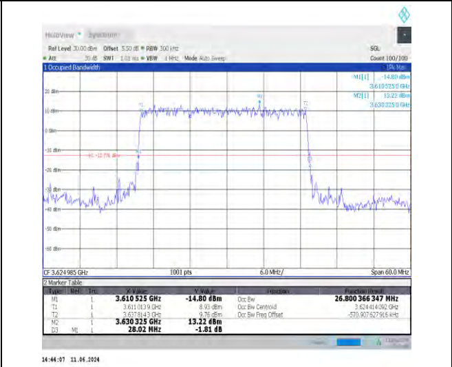
1-N48-30-30-M-2-DFT-PI2BPSK-Outer_Full-75@0-Ant0 -26.802-28.020-≤30-PASS
