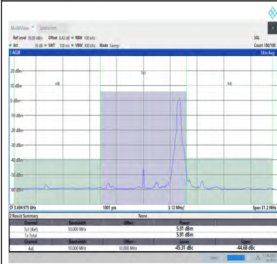
NTNV_N48_PC3_30_10_H_TID3_#1_-10_10
