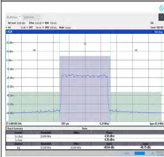
NTNV_N48_PC3_30_20_H_TID7 #1_-20_20
