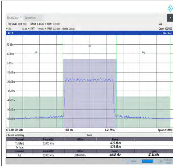
NTNV_N48_PC3_30_20_H_TID10_#1_-20_20
