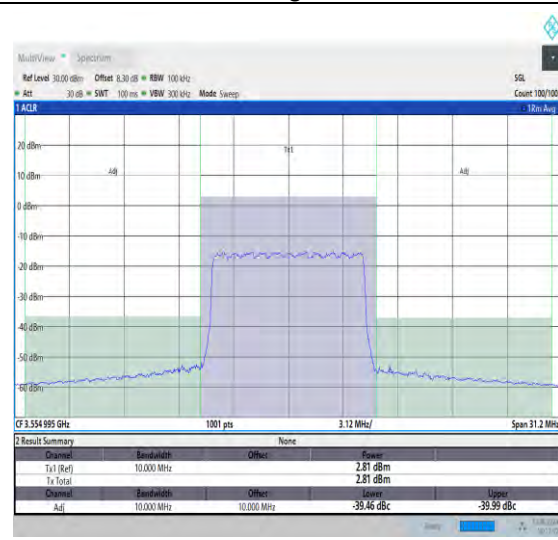
NTNV_N48_PC3_30_10_L_TID22_#1_-10_10
