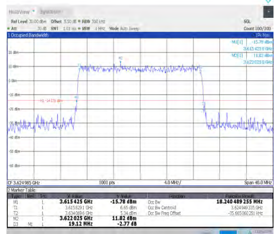
1-N48-30-20-M-7-CP-16QAM-Outer_Full-51@0-Ant 0-18.24-19.120-≤20-PASS
