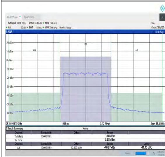
NTNV_N48_PC3_30_10_H_TID19_#1_-10_10
