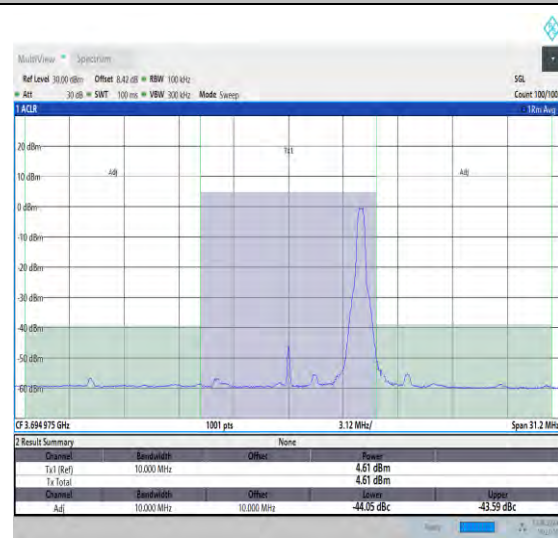
NTNV_N48_PC3_30_10_H_TID9_#1_-10_10
