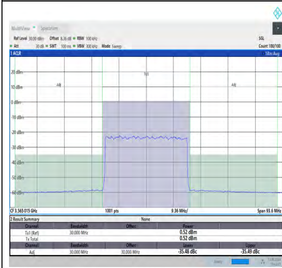
NTNV_N48_PC3_30_30_L_TID25_#1_-30_30
