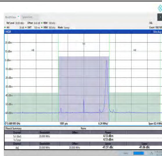
NTNV_N48_PC3_30_20_H_TID21_#1_-20_20
