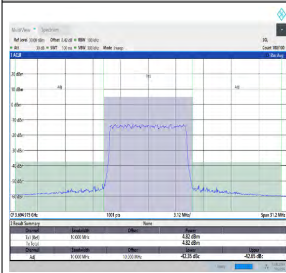
NTNV_N48_PC3_30_10_H_TID7_#1_-10_10
