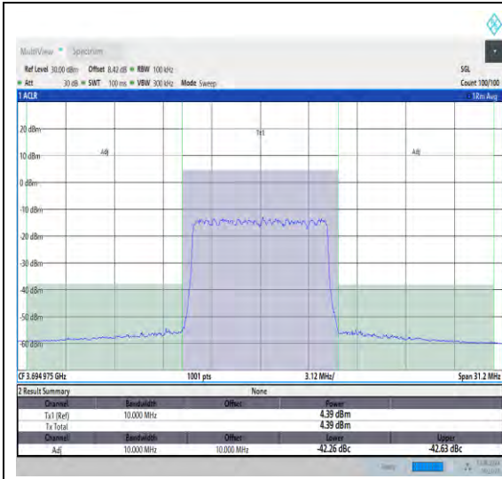
NTNV_N48_PC3_30_10_H_TID10_#1_-10_10
