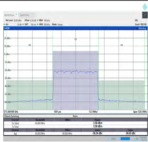
NTNV_N48_PC3_30_40_L_TID19_#1_-40_40
