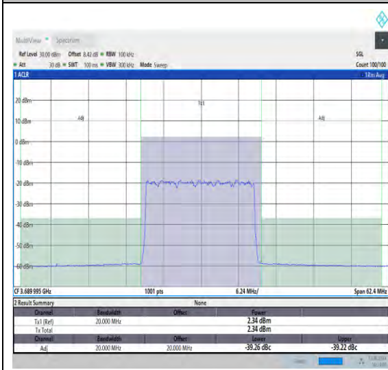
NTNV_N48_PC3_30_20_H_TID13_#1_-20_20
