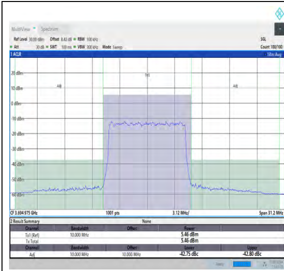
NTNV_N48_PC3_30_10_H_TID4_#1_+10_10
