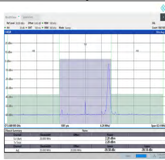
NTNV_N48_PC3_30_20_H_TID24_#1_-20_20
