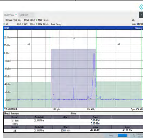
NTNV_N48_PC3_30_20_H_TID3_#1_-20_20
