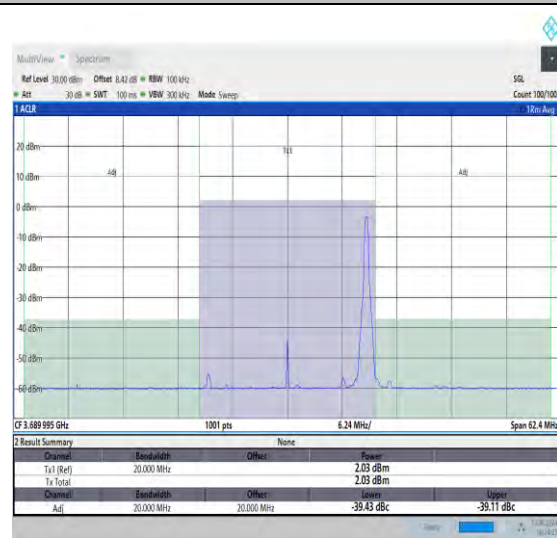
NTNV_N48_PC3_30_20_H_TID15_#1_-20_20
