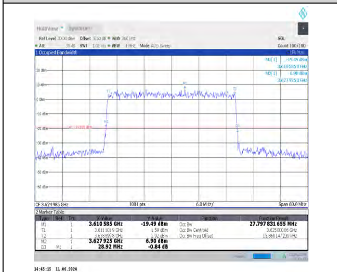
1-N48-30-30-M-9-CP-256QAM-Outer_Full-78@0-Ant0 0-27.8-28.920-≤30-PASS
