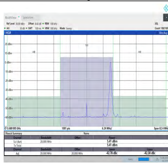
NTNV_N48_PC3_30_20_H_TID12_#1_-20_20
