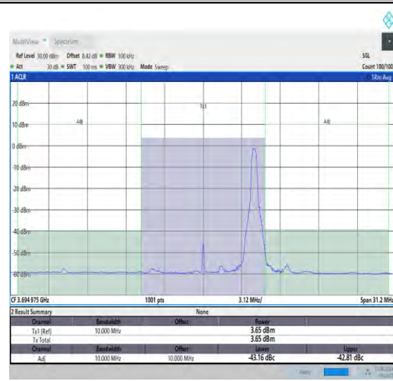
NTNV_N48_PC3_30_10_H_TID21_#1_-10_10
