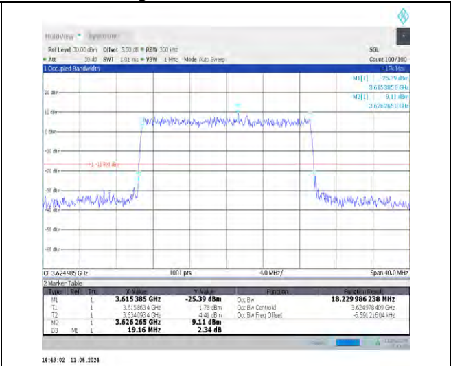
1-N48-30-20-M-9-CP-256QAM-Outer_Full-51@0-Ant0 -18.23-19.160-≤20-PASS
