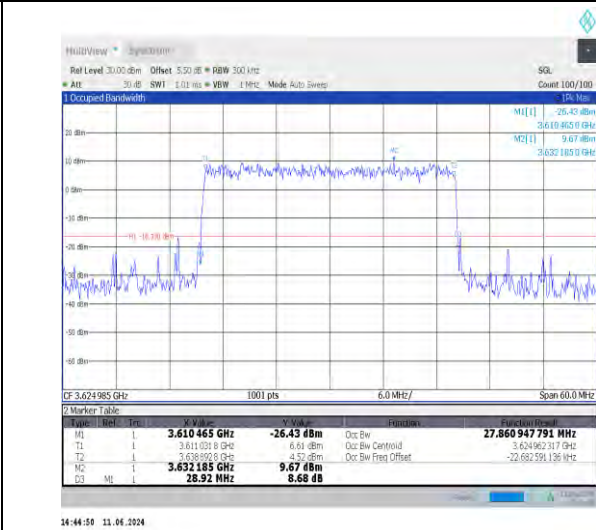
1-N48-30-30-M-6-CP-QPSK-Outer_Full-78@0-Ant0 27.861-28.920-≤30-PASS
