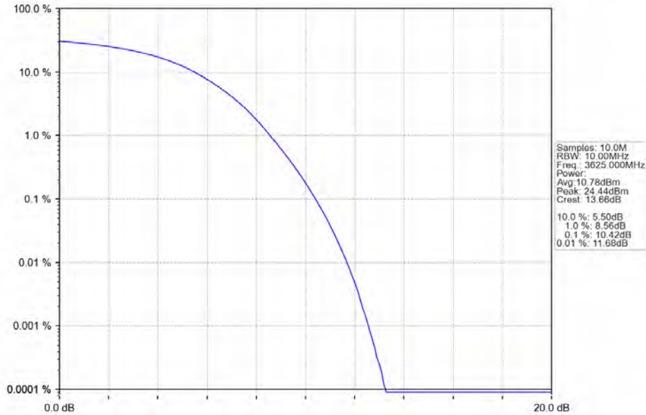
Band48_5MHz_256QAM_MCH_3625MHz_RB_25_0_NTNV
