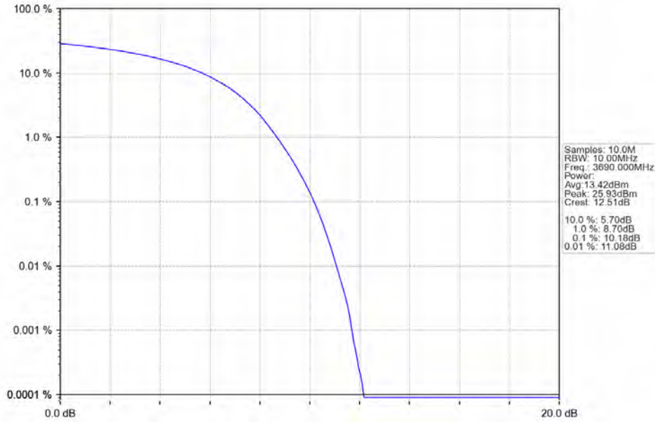
Band48_20MHz_64QAM_HCH_3690MHz_RB_100_0_NTNV
