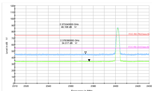
Bluetooth LE (S=2) Channel 0 Peak+ Average
