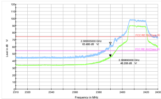
802.11g-Channel 1 Peak+ Average
