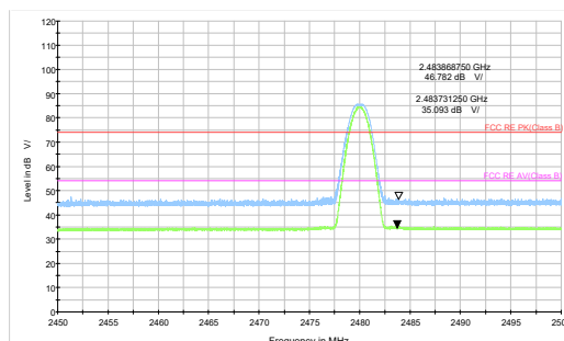
Bluetooth LE (S=2) Channel 39 Peak+Average
