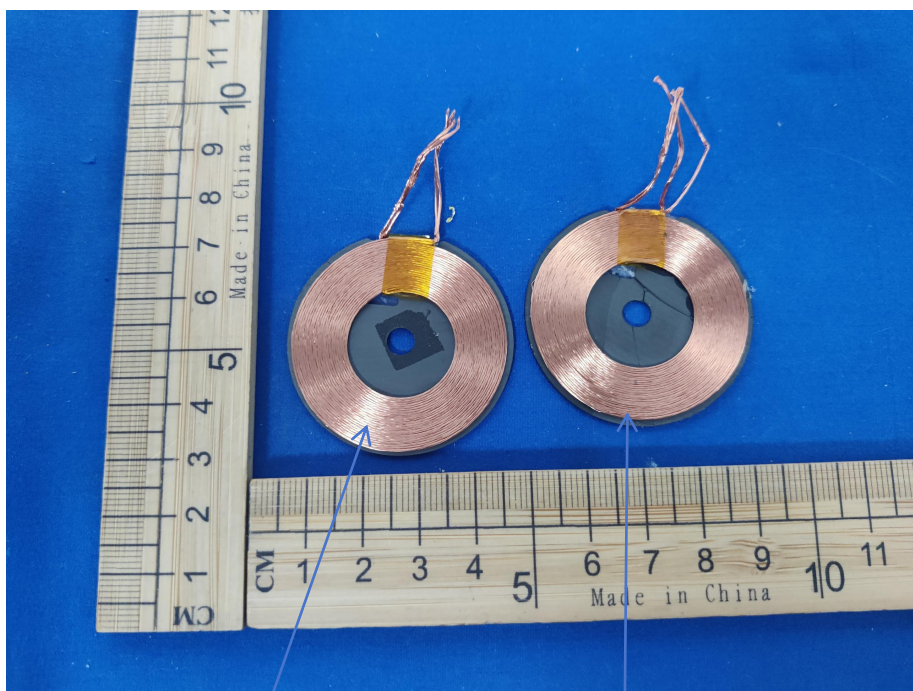
ANT 1 Transmitting coil
