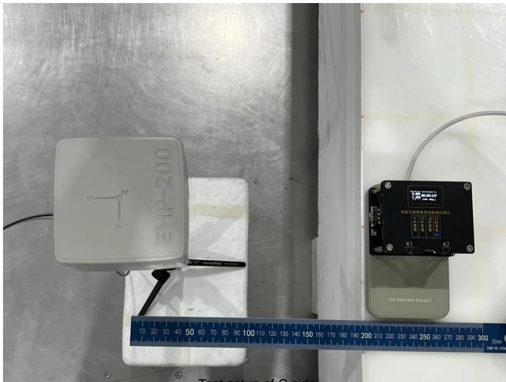
Test setup of C side
