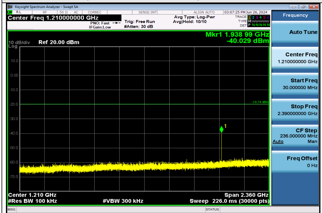
Test_Graph_LE1M_ANT1_2402_1Mbps_Lower Band Emissions
