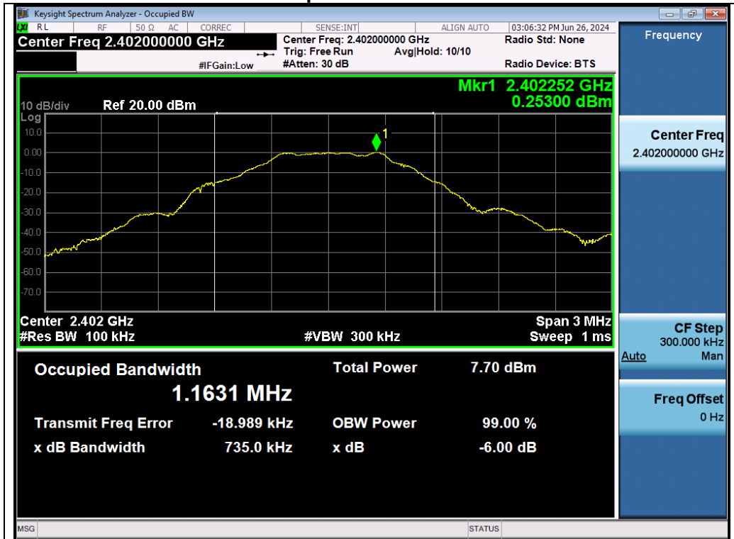
Test_Graph_LE1M_ANT1_2402_1Mbps_DTSSBW
