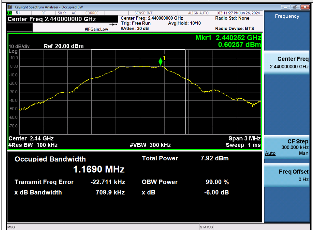
Test_Graph_LE1M_ANT1_2440_1Mbps_DTSSBW
