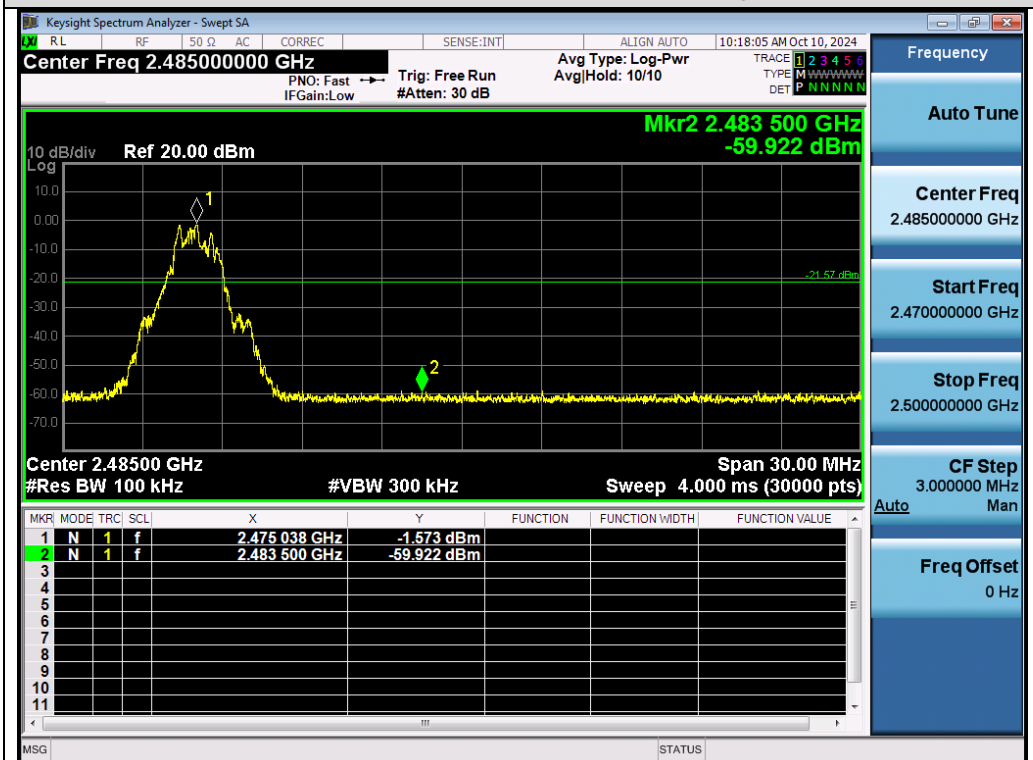
Test_Graph_2.4G_ANT1_2475_Higher Band Edge Emissions
