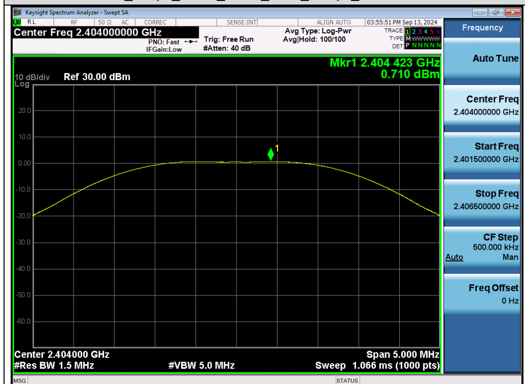
Test_Graph_LE2M_ANT1_2404_2Mbps_Peak Power
