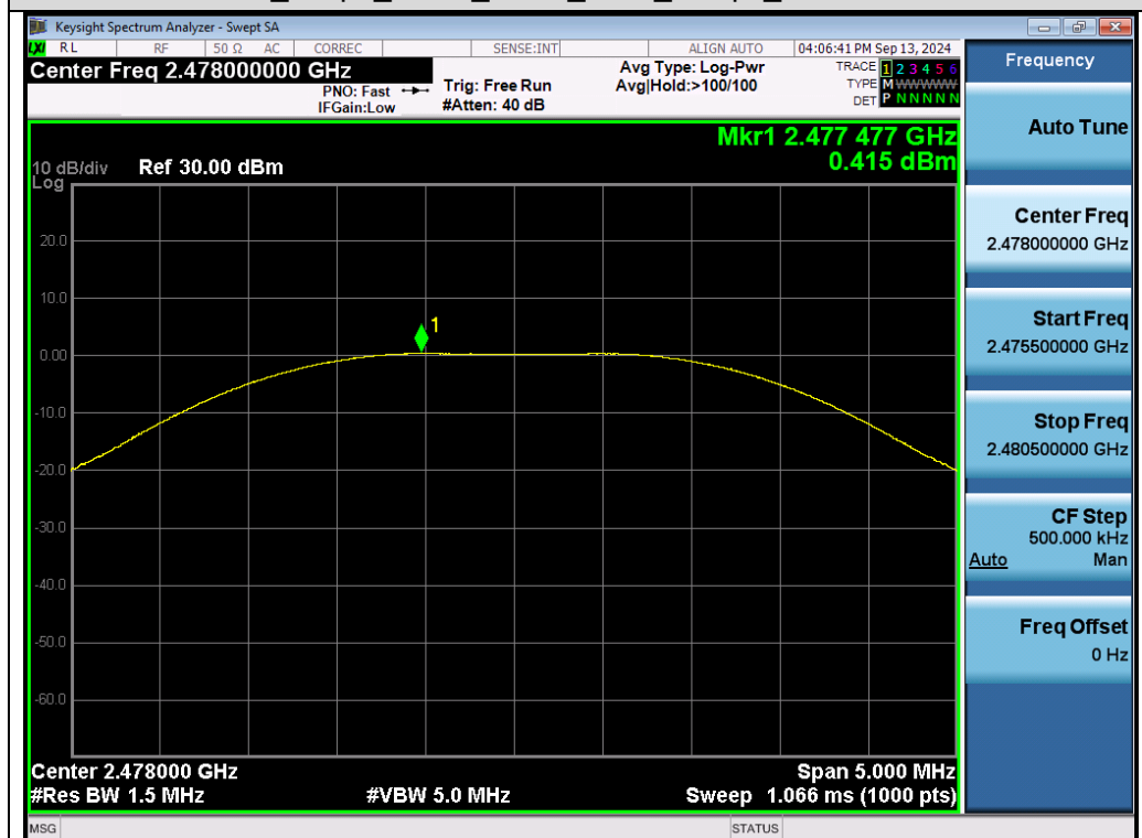
Test_Graph_LE2M_ANT1_2478_2Mbps_Peak Power
