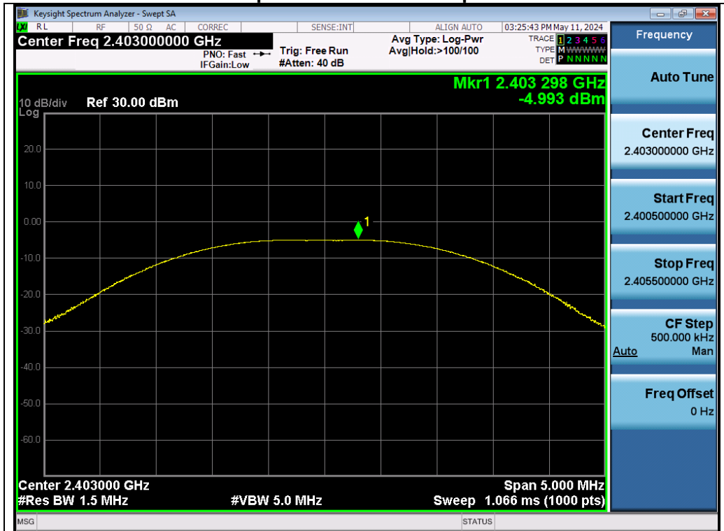
Test_Graph_GFSK_ANT1_2403_Peak Power
