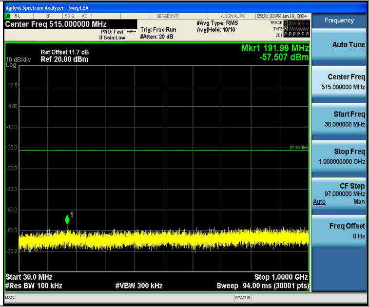
BLE_1M-Ant1-2480-30~1000-PASS
