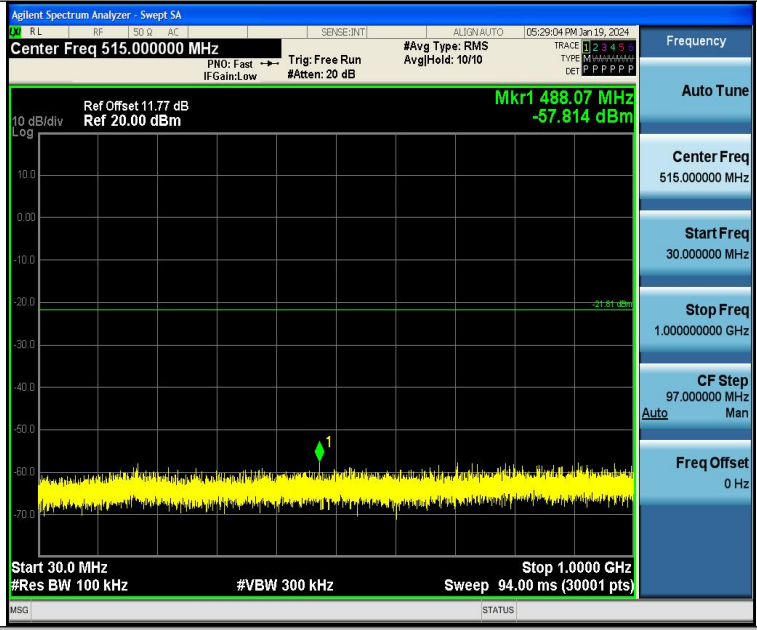
BLE_1M-Ant1-2440-30~1000-PASS
