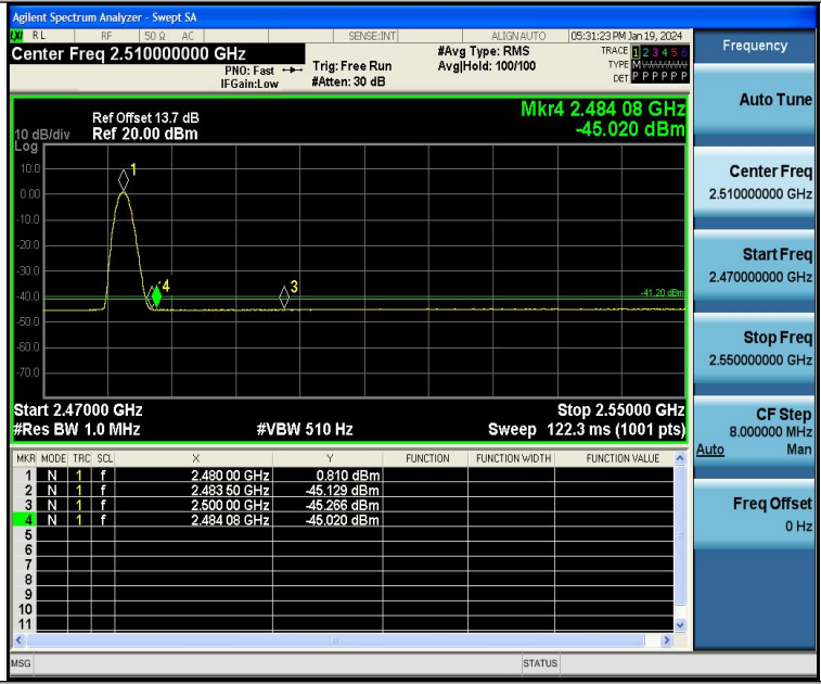
BLE_1M-Ant1-2480-PASS
