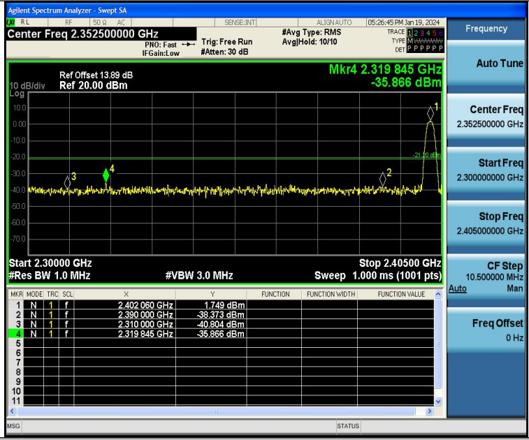
BLE_1M-Ant1-2402-PASS
