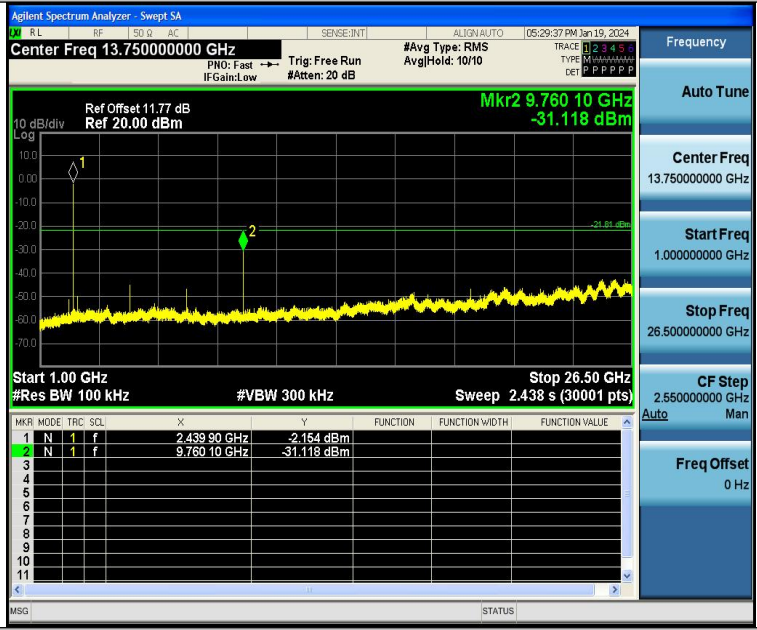
BLE_1M-Ant1-2440-1000~26500-PASS
