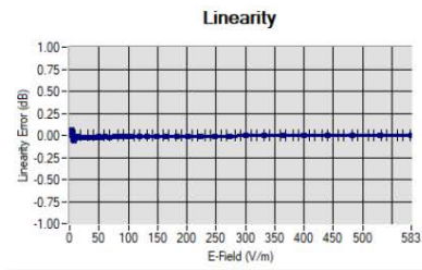
Linearity: +/-1.43% (+/-0.06dB)
