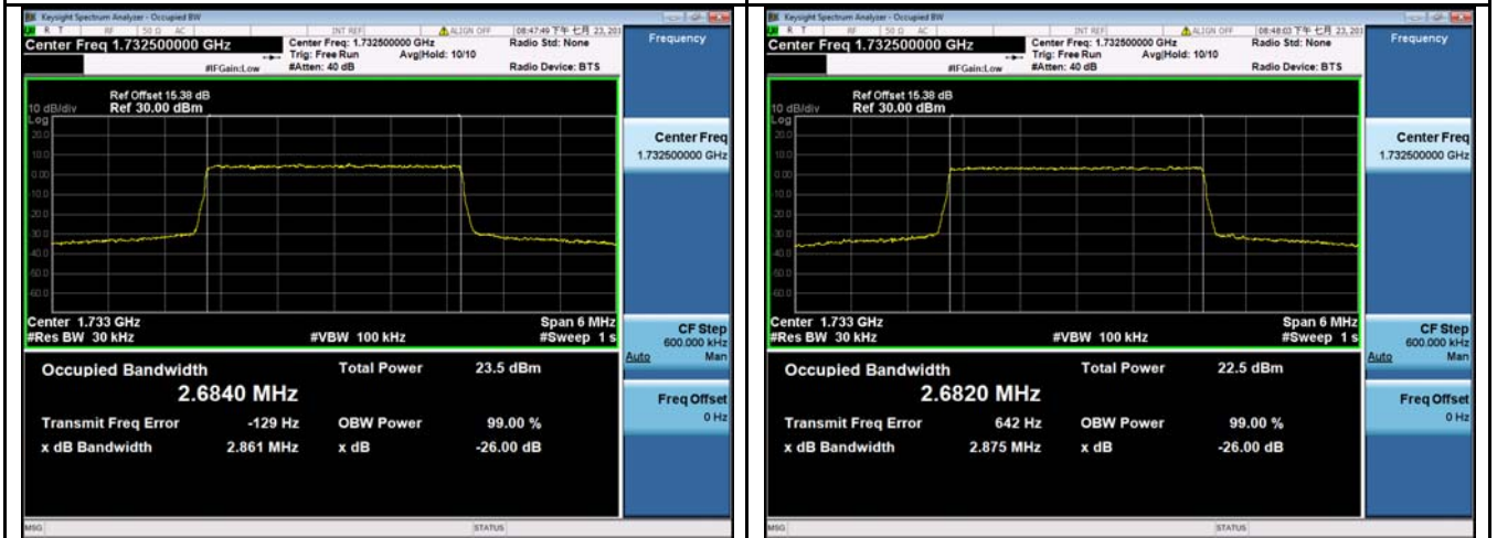
LTE band 4 - Middle CH QPSK-3
