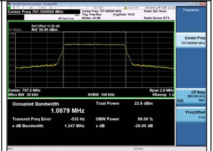
LTE band 12 - Middle CH 16QAM-1.4
