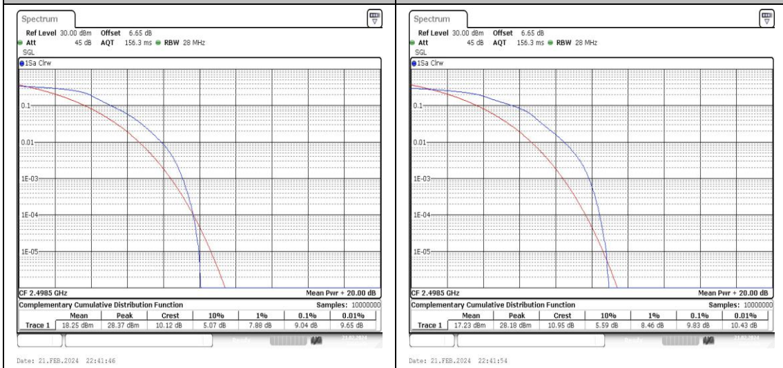
Band41-5MHz-QPSK-39675-25RB#0-PASS Band41-5MHz-16QAM-39675-25RB#0-PASS
