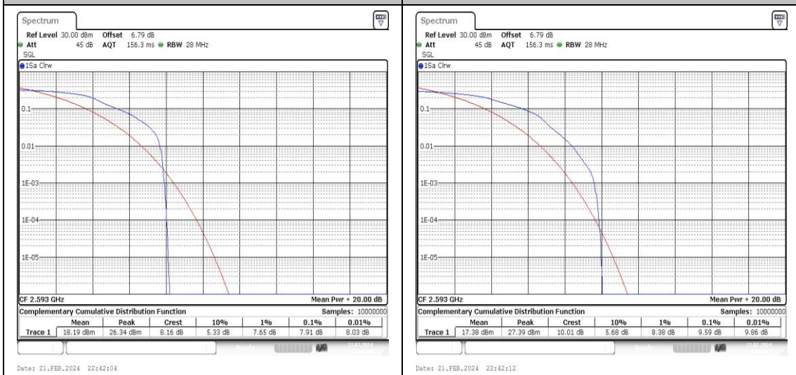
Band41-5MHz-QPSK-40620-1RB#0-PASS Band41-5MHz-16QAM-40620-1RB#0-PASS
