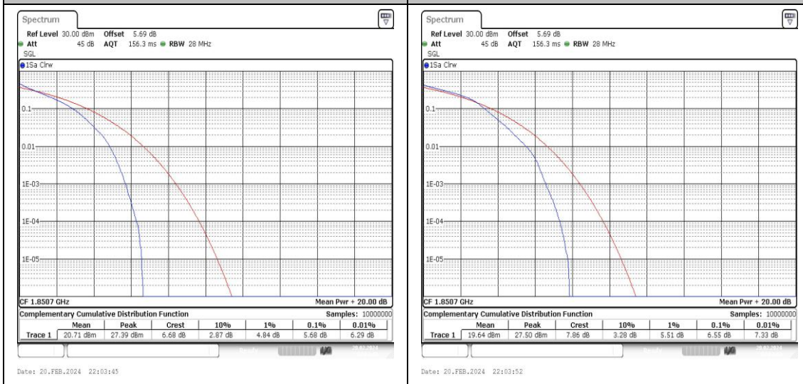
Band25-1.4MHz-QPSK-26047-6RB#0-PASS Band25-1.4MHz-16QAM-26047-6RB#0-PASS
