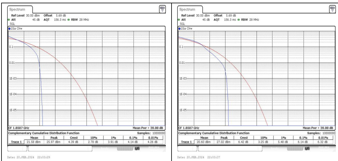
Band25-1.4MHz-QPSK-26047-1RB#0-PASS Band25-1.4MHz-16QAM-26047-1RB#0-PASS
