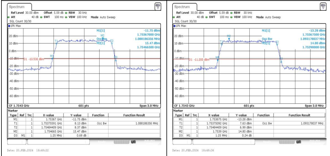
Band4-1.4MHz-QPSK-20175-6RB#0-PASS
