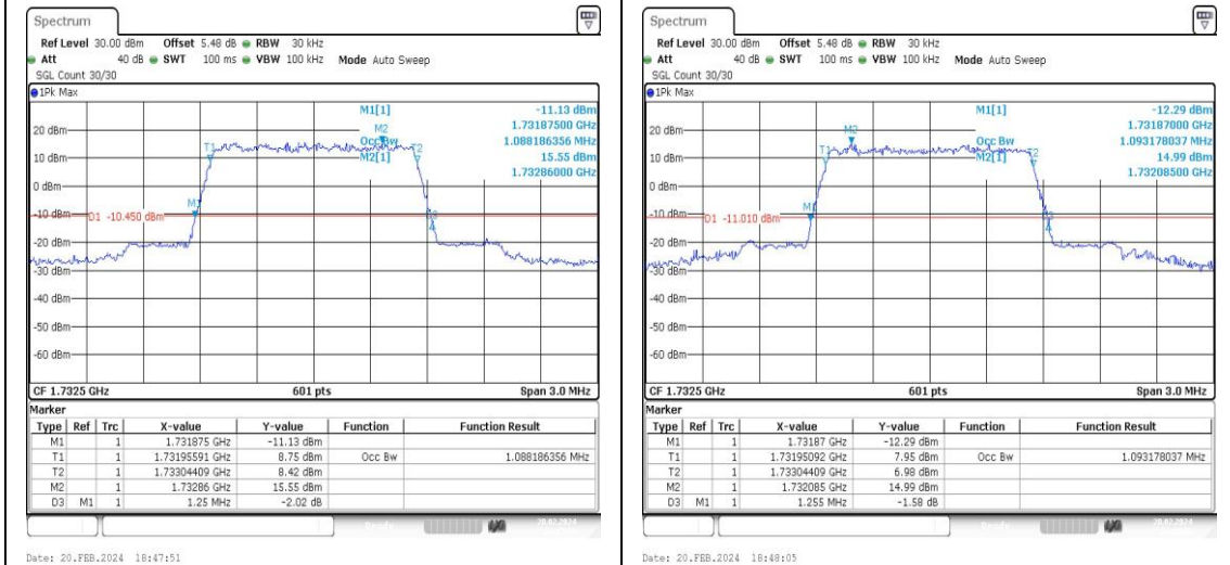
Band4-1.4MHz-QPSK-20175-6RB#0-PASS
