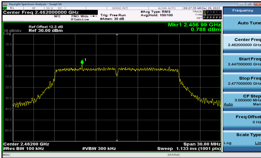
11N20SISO-Ant1-2462-0~Reference-PASS
