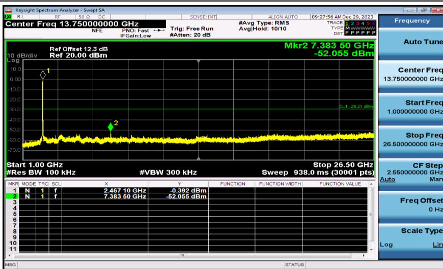
11N20SISO-Ant1-2462-1000~26500-PASS
