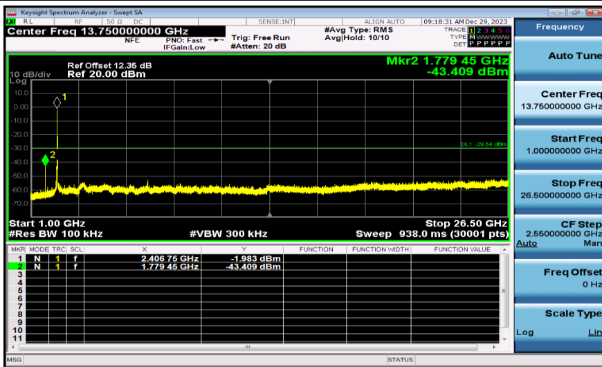
11N20SISO-Ant1-2412-1000~26500-PASS
