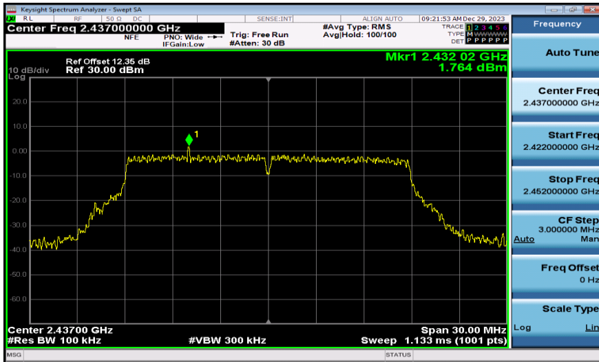
11N20SISO-Ant1-2437-0~Reference-PASS
