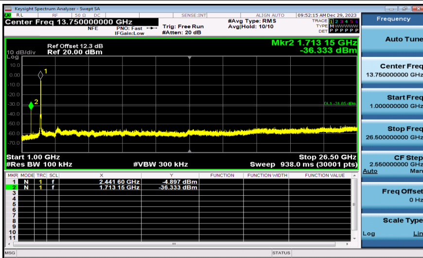
11N40SISO-Ant1-2452-1000~26500-PASS
