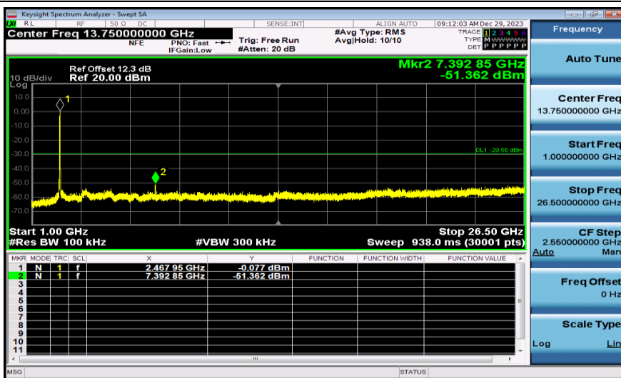
11G-Ant1-2462-1000~26500-PASS
