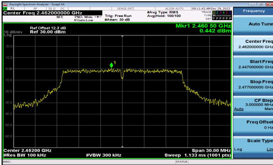
11G-Ant1-2462-0~Reference-PASS
