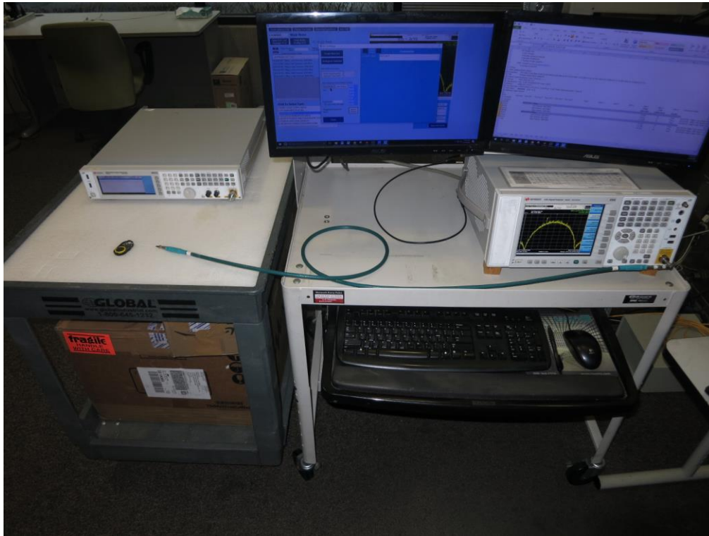
Direct Connect
