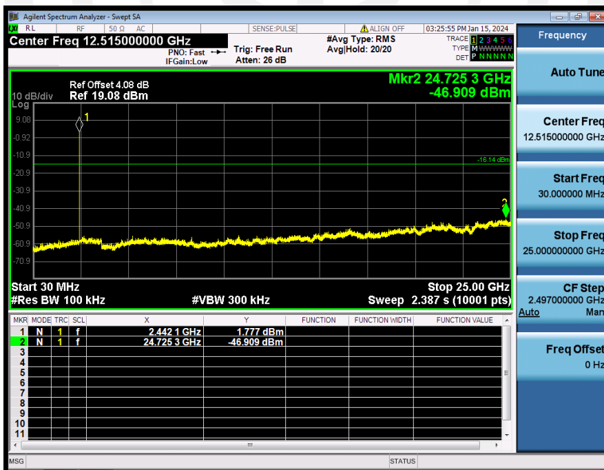
Spurious_Emissions_NVNT_ANT1_1-DH1_2441
