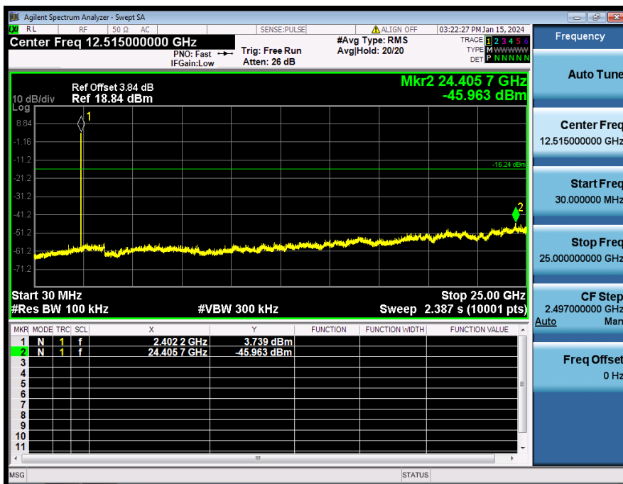
Spurious_Emissions_NVNT_ANT1_1-DH1_2402
