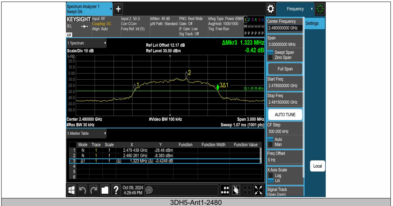
3DH5-Ant1-2480
