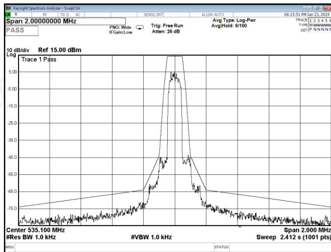
Channel 16 / 535.1 MHz
