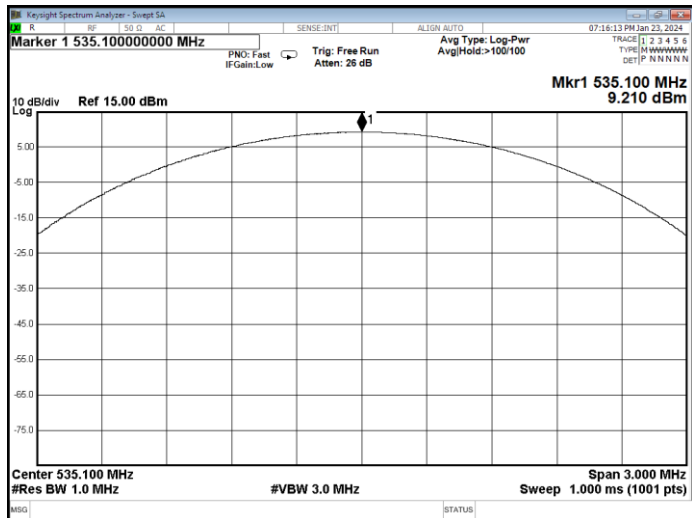
Channel 16 / 535.1 MHz
