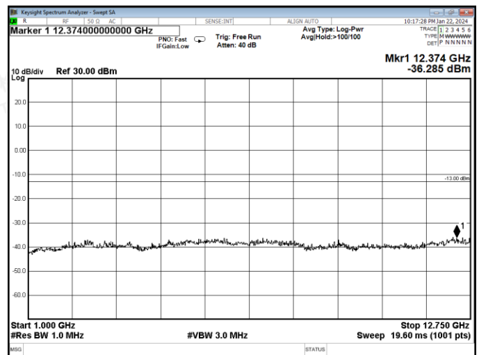
Channel 16 / 535.1 MHz
