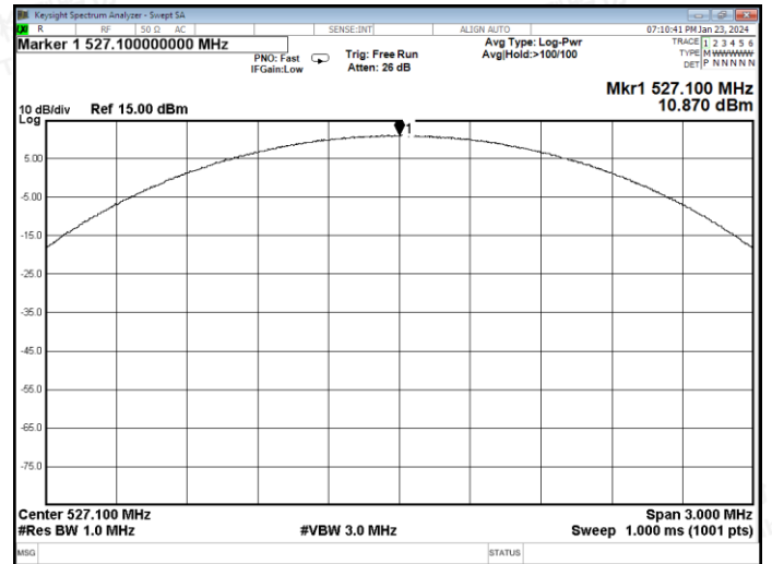
Channel 8 / 527.1 MHz
