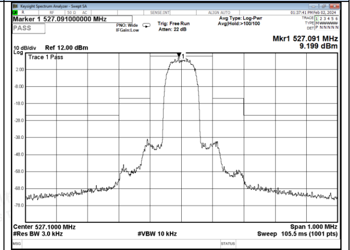
Channel 8 / 527.1 MHz
