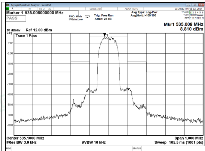
Channel 16 / 535.1 MHz
