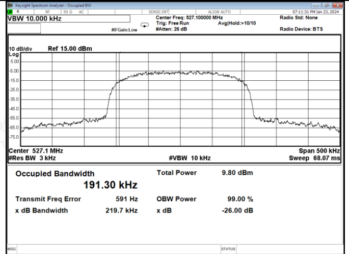
Channel 8 / 527.1 MHz
