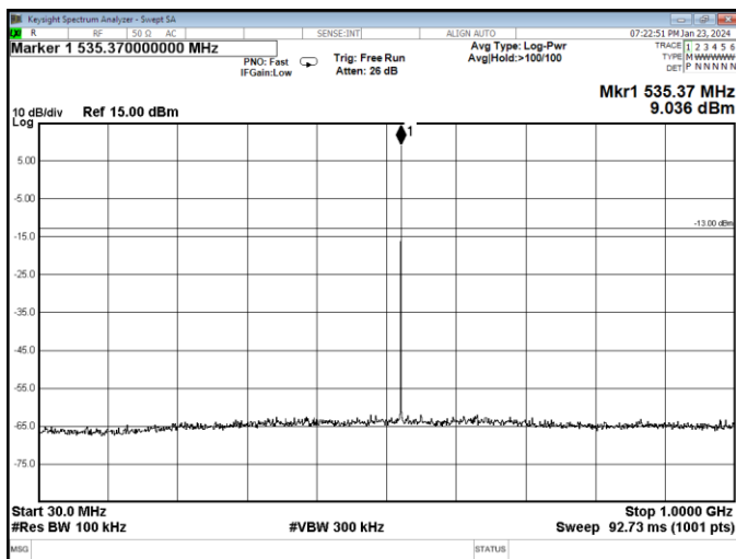
Channel 16 / 535.1 MHz
