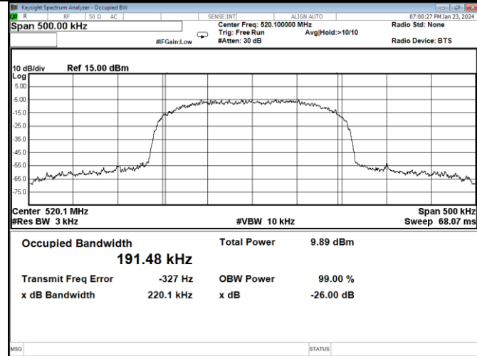
Channel 1 / 520.1 MHz
