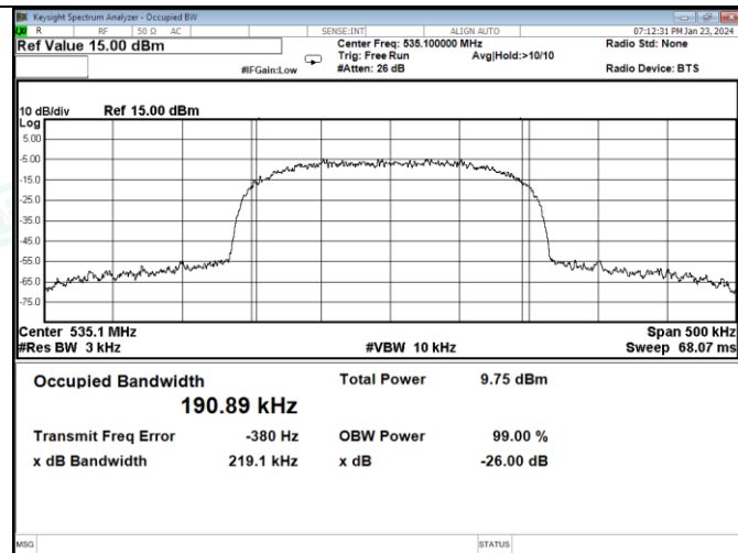
Channel 16 / 535.1 MHz
