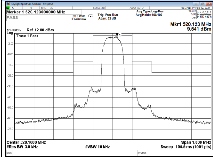
Channel 1 / 520.1 MHz
