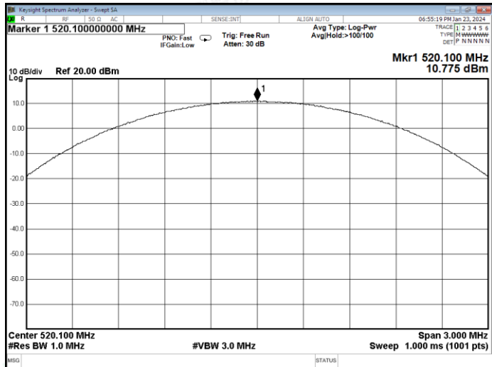
Channel 1 / 520.1 MHz
