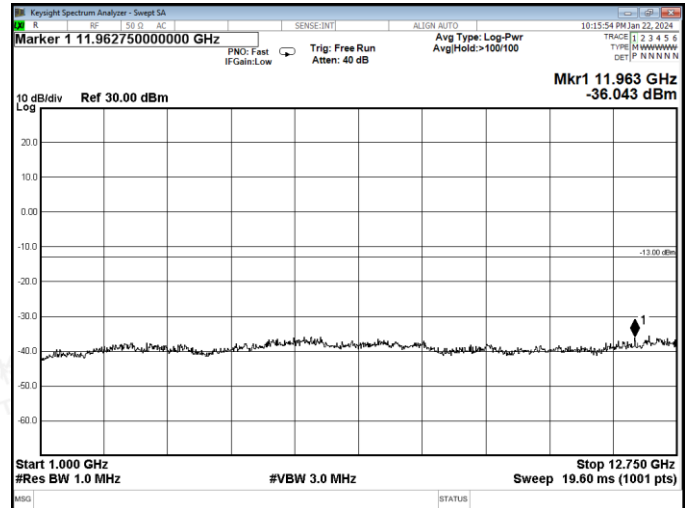
Channel 1 / 520.1 MHz
