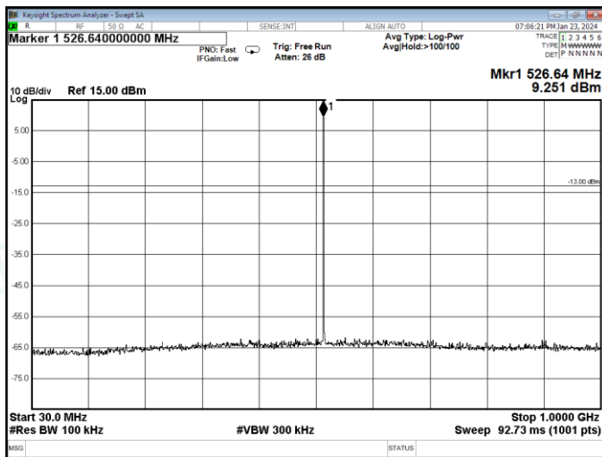
Channel 8 / 527.1 MHz
