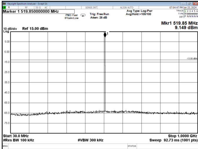
Channel 1 / 520.1 MHz
