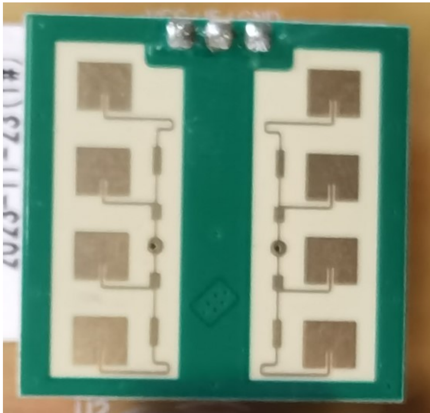
Photo 19— antenna of 24GHz RF Module
