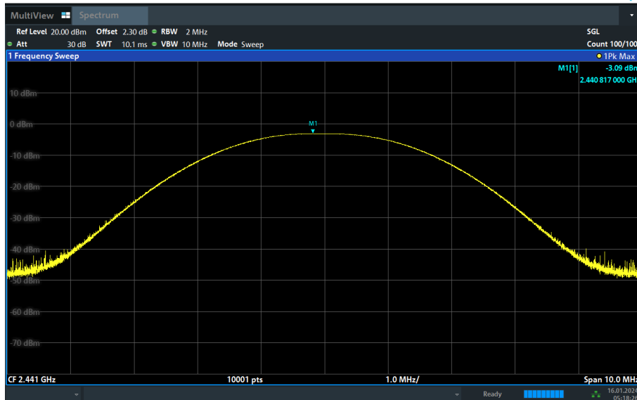
GFSK mode-CH39
