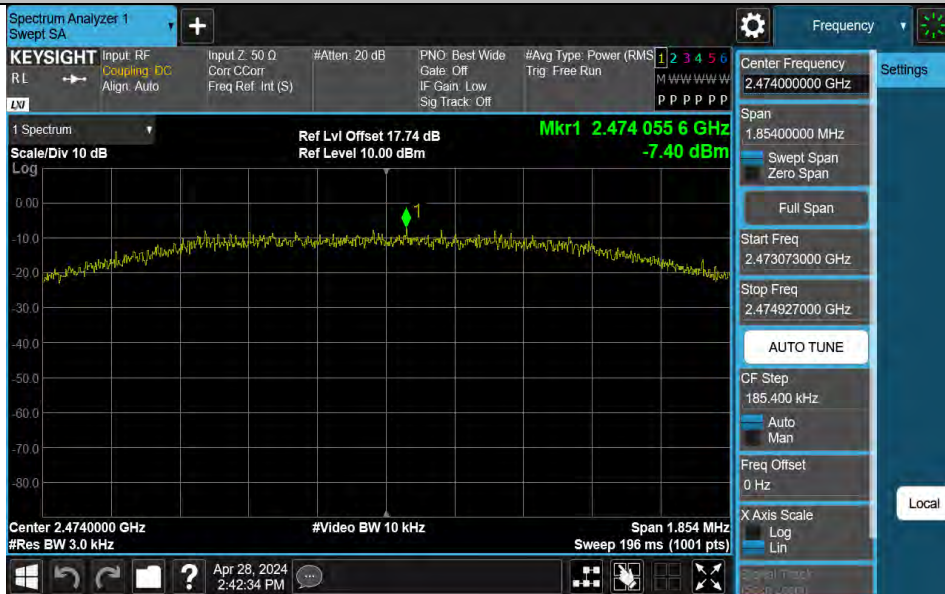
GFSK-Ant1-2474-PASS
