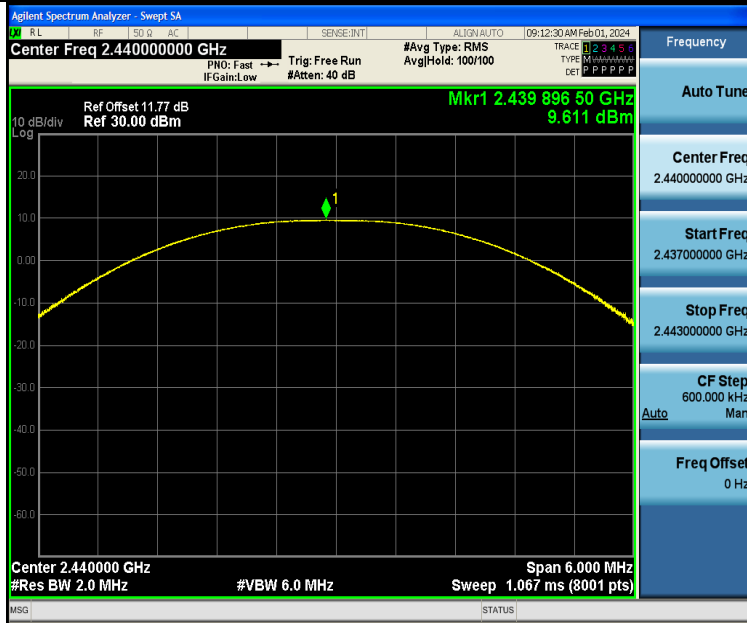
BLE_1M-Ant2-2440-PASS
