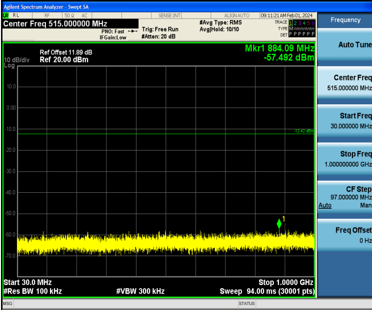
BLE_1M-Ant2-2402-30~1000-PASS
