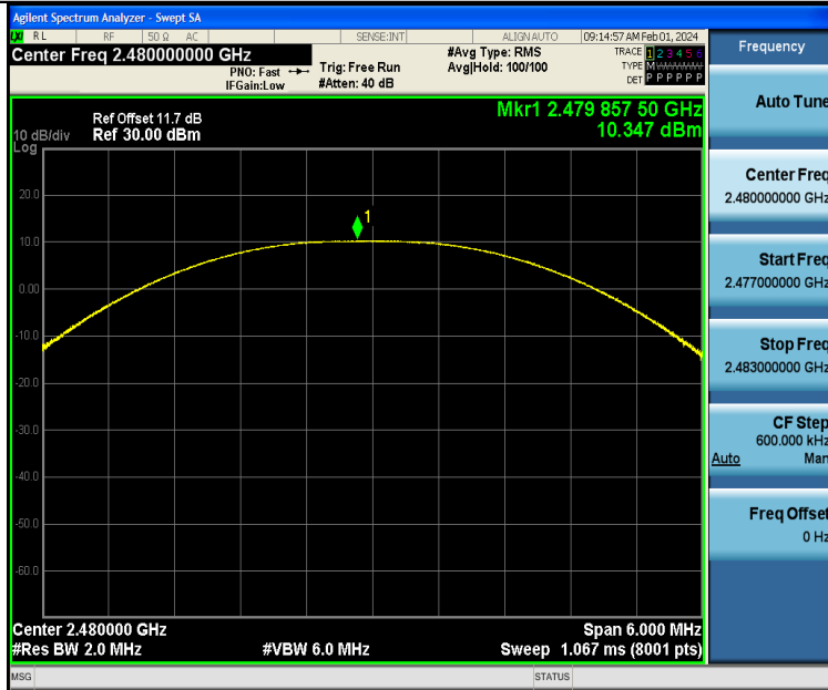
BLE_1M-Ant2-2480-PASS
