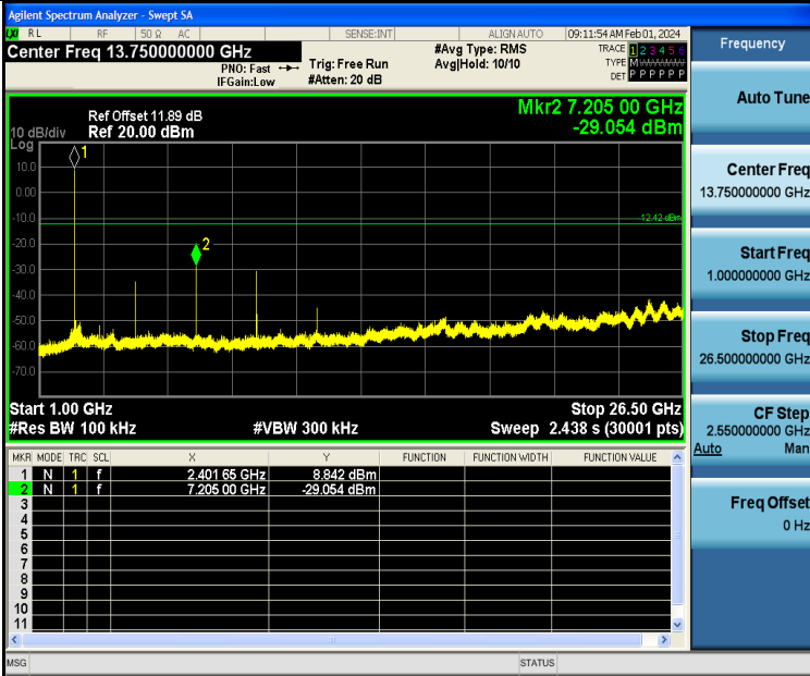
BLE_1M-Ant2-2402-1000~26500-PASS
