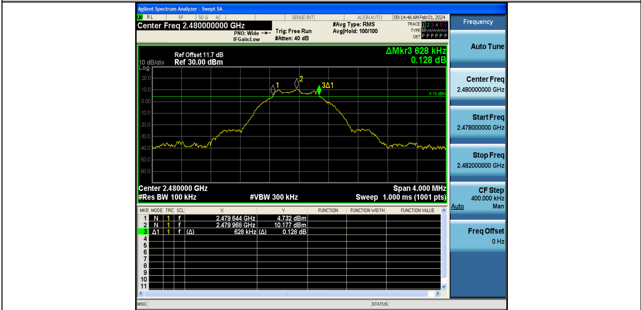
BLE_1M-Ant2-2480-PASS
