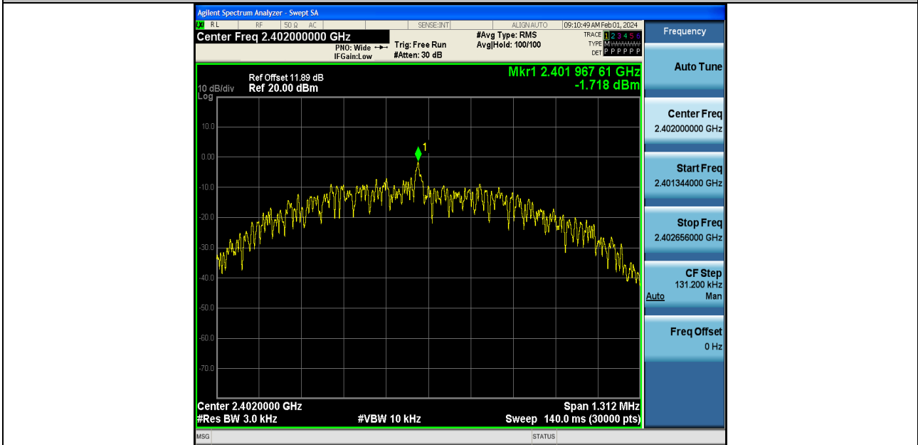
BLE_1M-Ant2-2402-PASS
