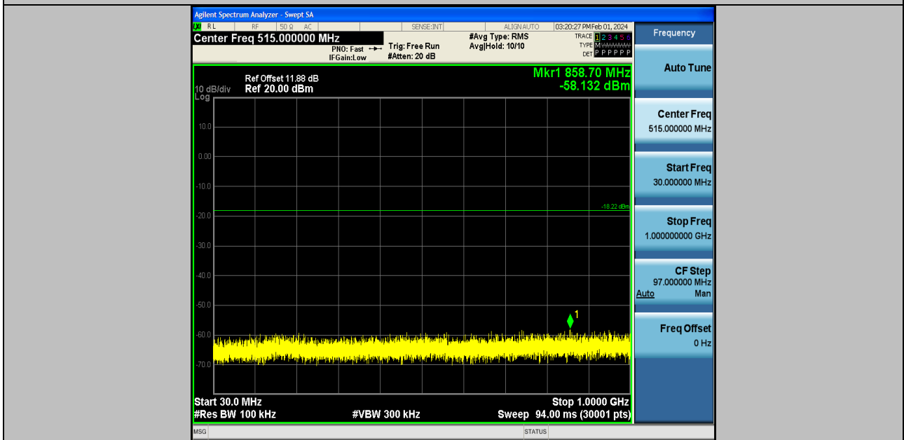
3DH5-Ant2-2441-30~1000-PASS
