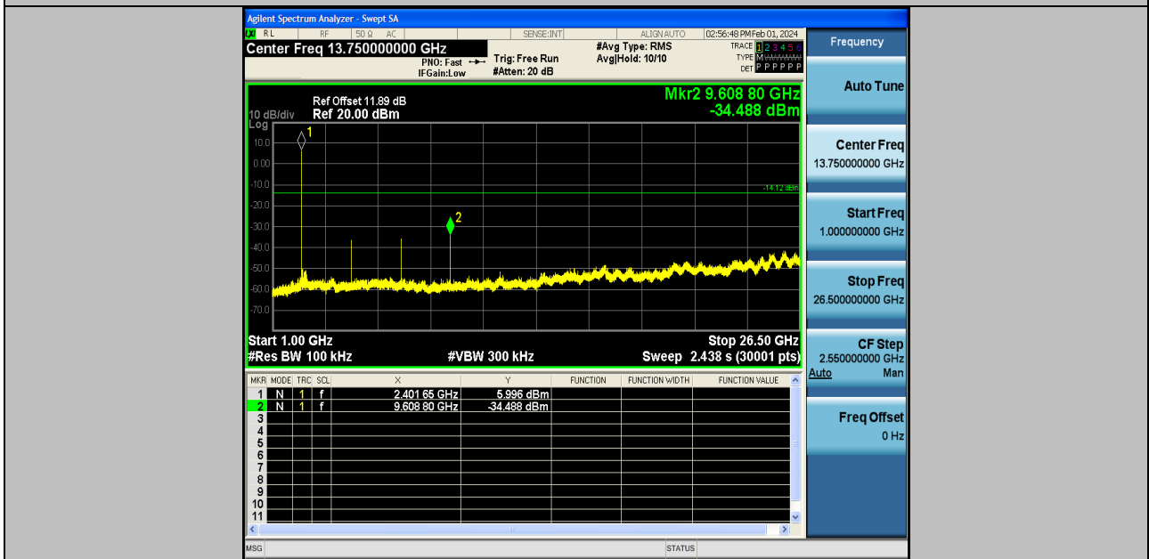
DH5-Ant2-2402-1000~26500-PASS
