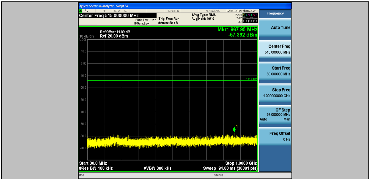
DH5-Ant2-2402-30~1000-PASS
