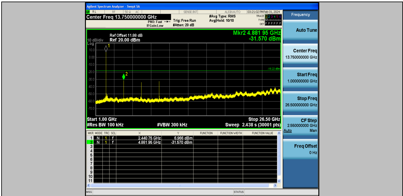
3DH5-Ant2-2441-1000~26500-PASS
