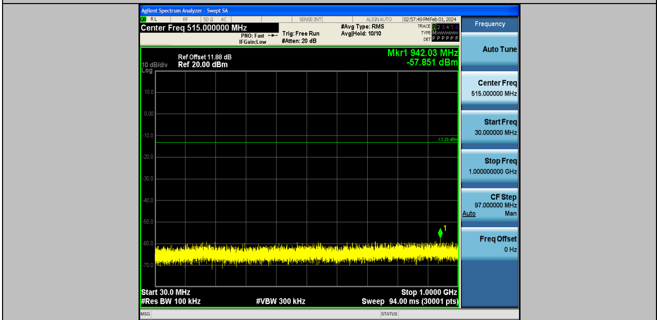
DH5-Ant2-2441-30~1000-PASS
