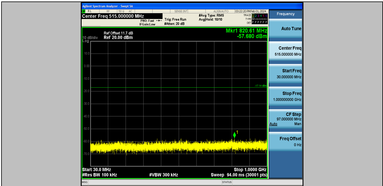
3DH5-Ant2-2480-30~1000-PASS
