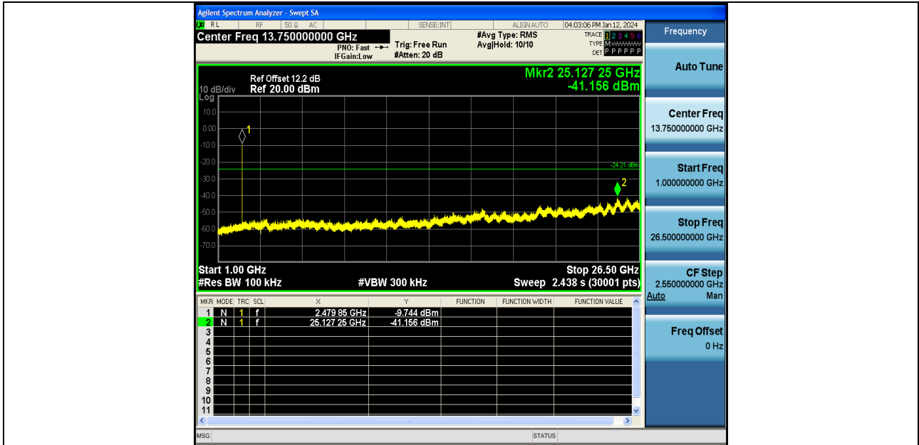
3DH5-Ant1-2480-1000~26500-PASS
