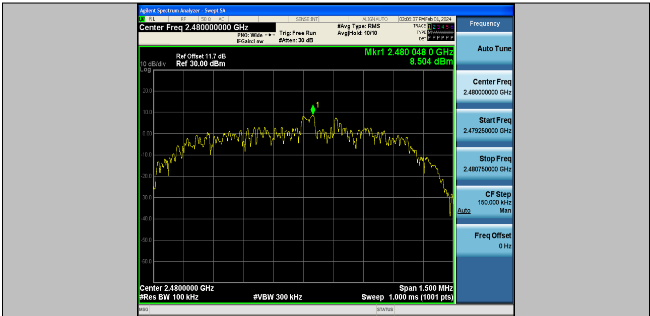
2DH5-Ant2-2480-0~Reference-PASS
