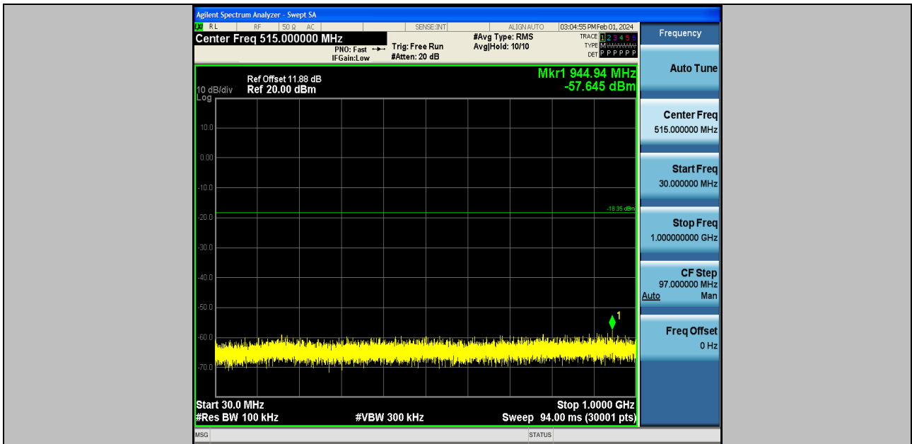
2DH5-Ant2-2441-30~1000-PASS
