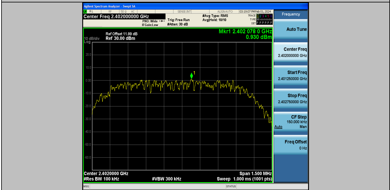
3DH5-Ant2-2402-0~Reference-PASS
