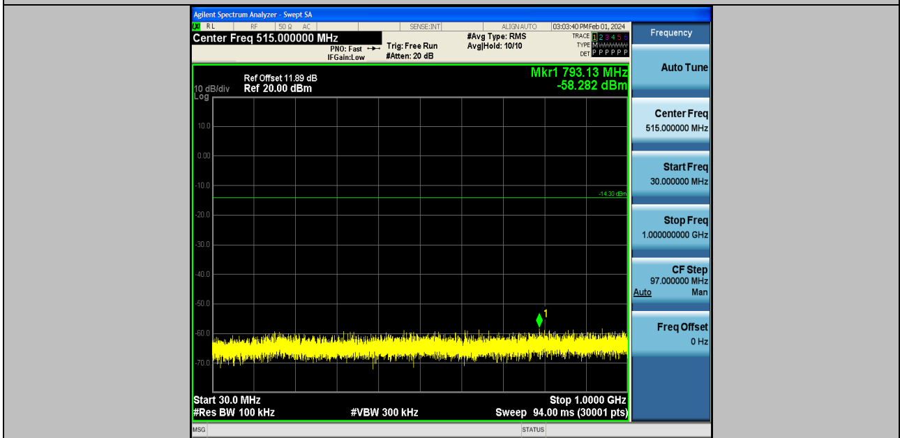
2DH5-Ant2-2402-30~1000-PASS
