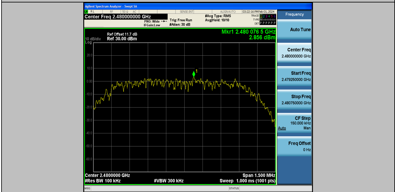
3DH5-Ant2-2480-0~Reference-PASS
