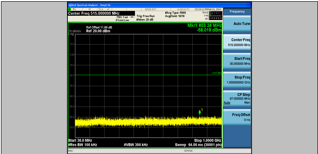
3DH5-Ant2-2402-30~1000-PASS
