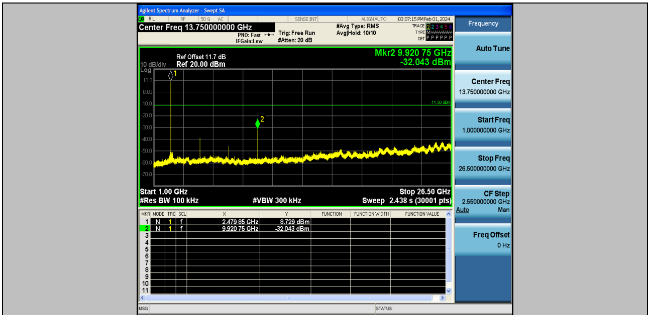
2DH5-Ant2-2480-1000~26500-PASS
