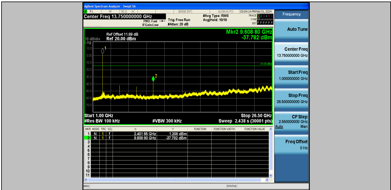
2DH5-Ant2-2402-1000~26500-PASS
