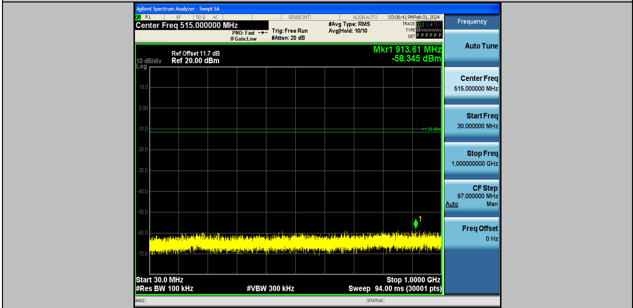
2DH5-Ant2-2480-30~1000-PASS
