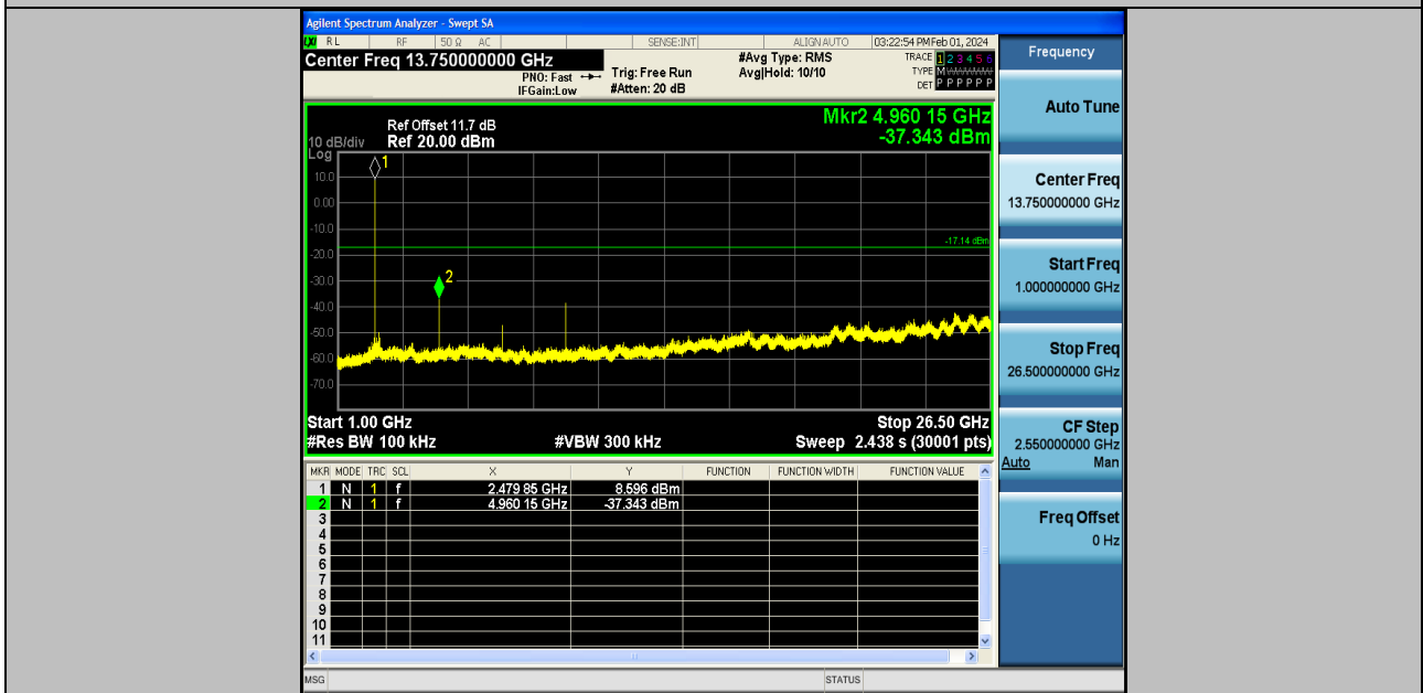
3DH5-Ant2-2480-1000~26500-PASS
