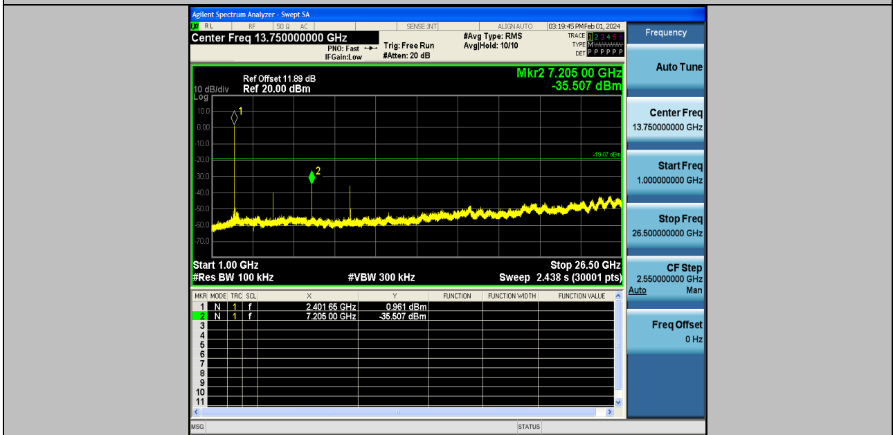
3DH5-Ant2-2402-1000~26500-PASS
