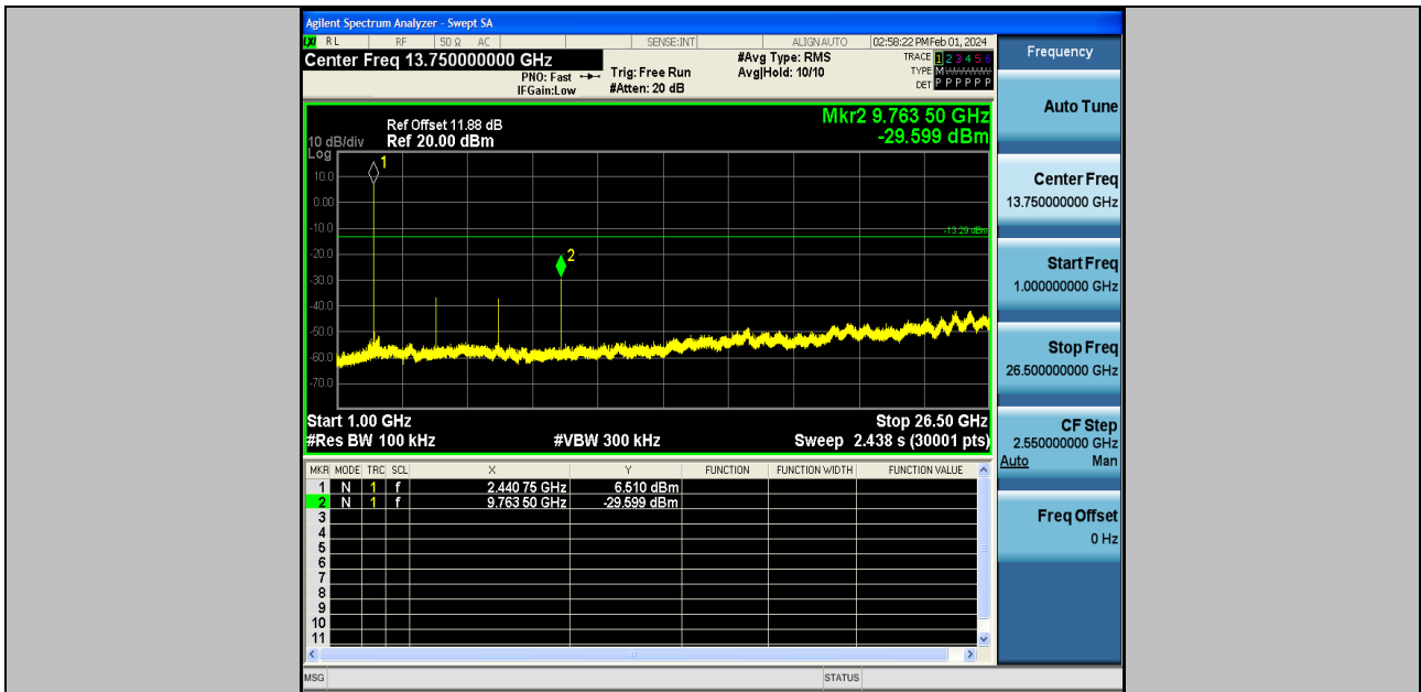
DH5-Ant2-2441-1000~26500-PASS
