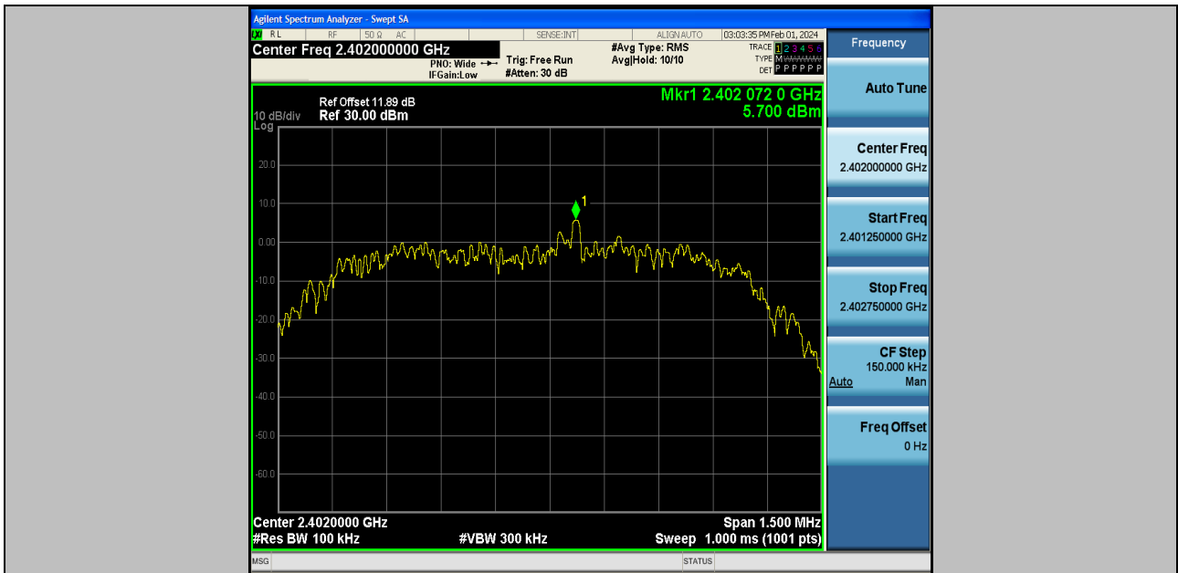
2DH5-Ant2-2402-0~Reference-PASS
