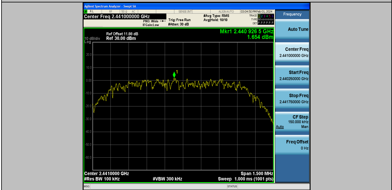
2DH5-Ant2-2441-0~Reference-PASS
