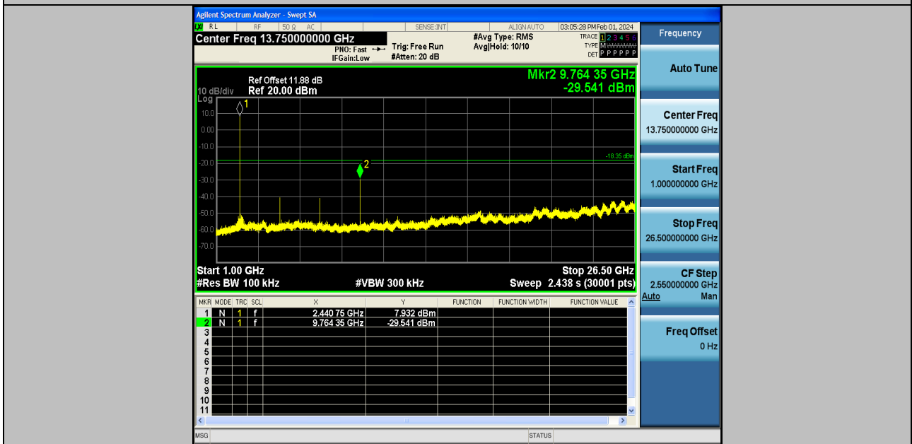
2DH5-Ant2-2441-1000~26500-PASS
