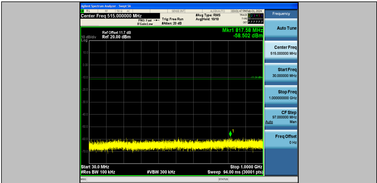
DH5-Ant2-2480-30~1000-PASS
