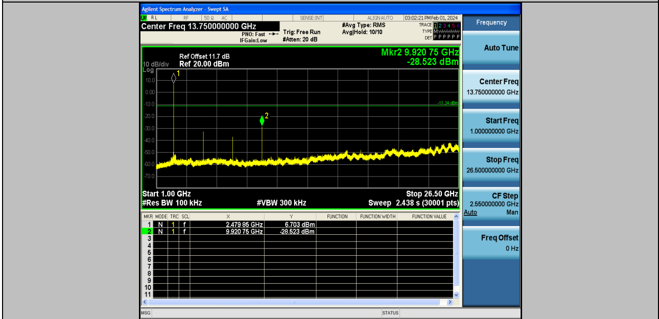
DH5-Ant2-2480-1000~26500-PASS
