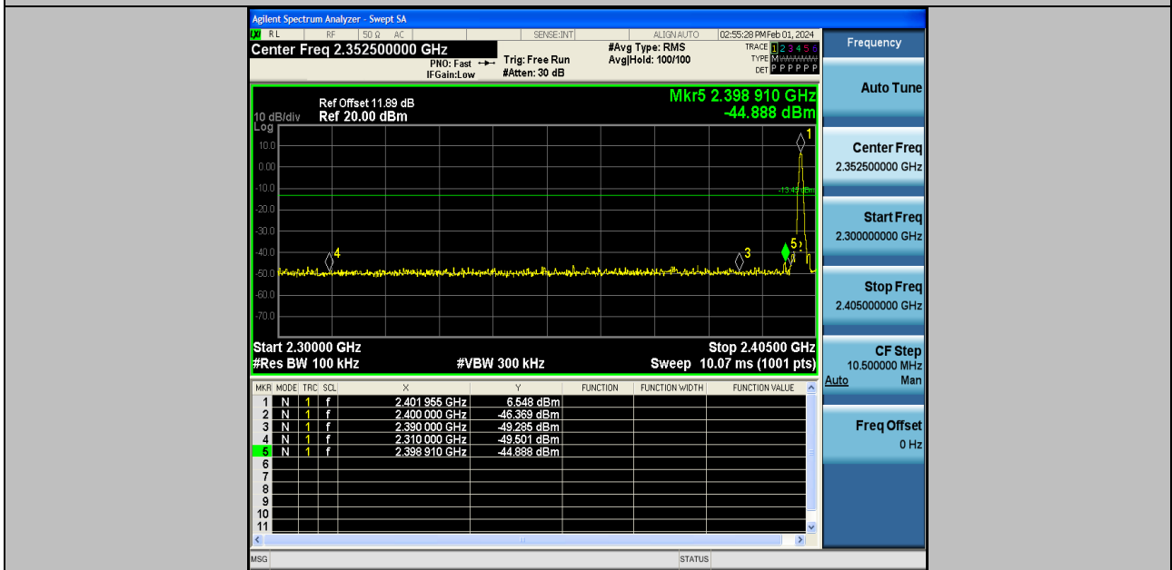
DH5-Ant2-2402-PASS
