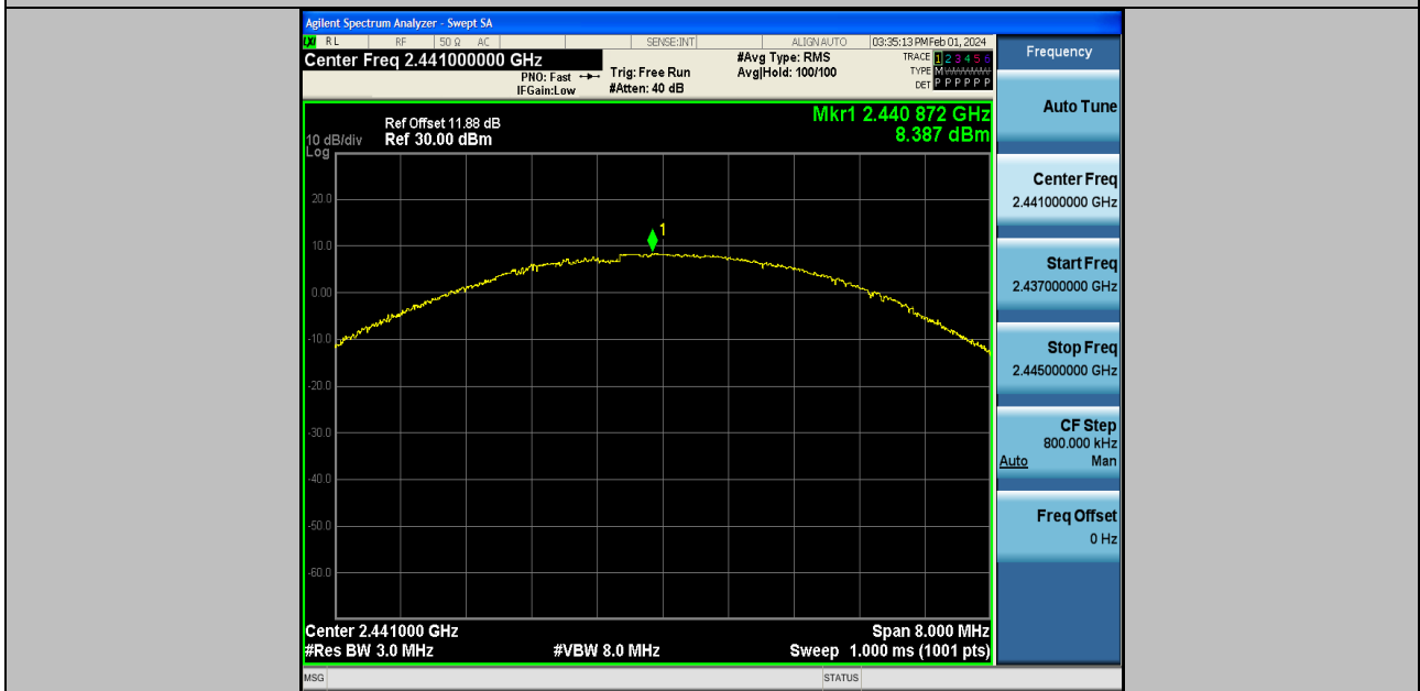
2DH5-Ant2-2441-PASS
