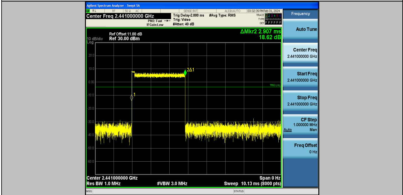
3DH5-Ant2-Hop-PASS
