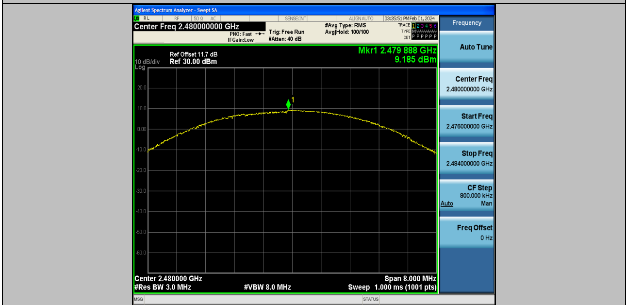
3DH5-Ant2-2480-PASS
