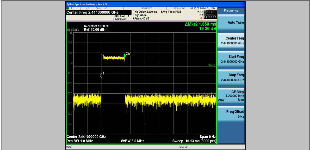
2DH3-Ant2-Hop-PASS
