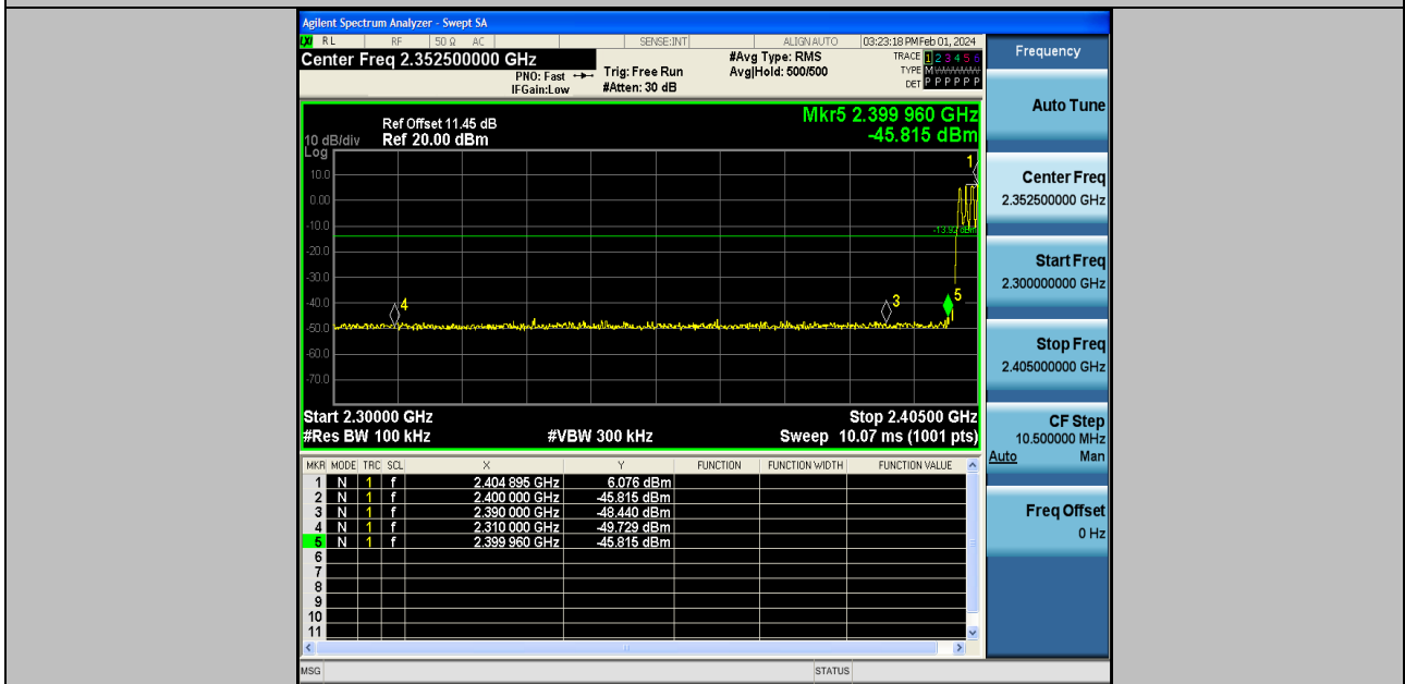
DH5-Ant2-Hop_2402-PASS
