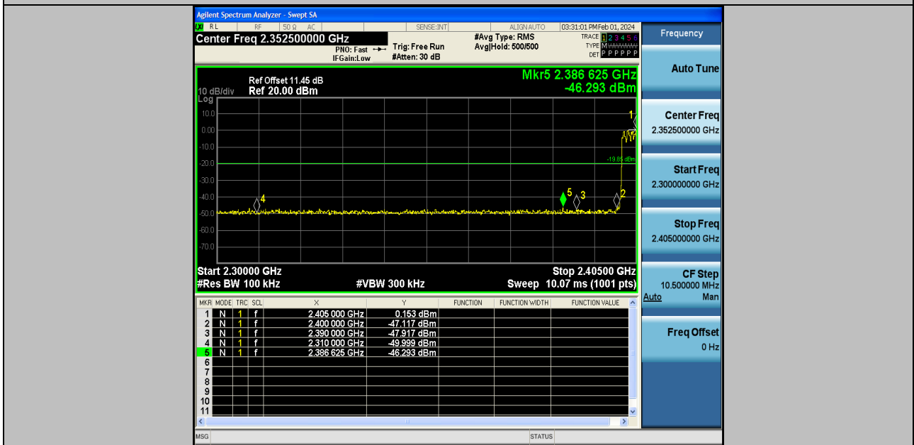
3DH5-Ant2-Hop_2402-PASS
