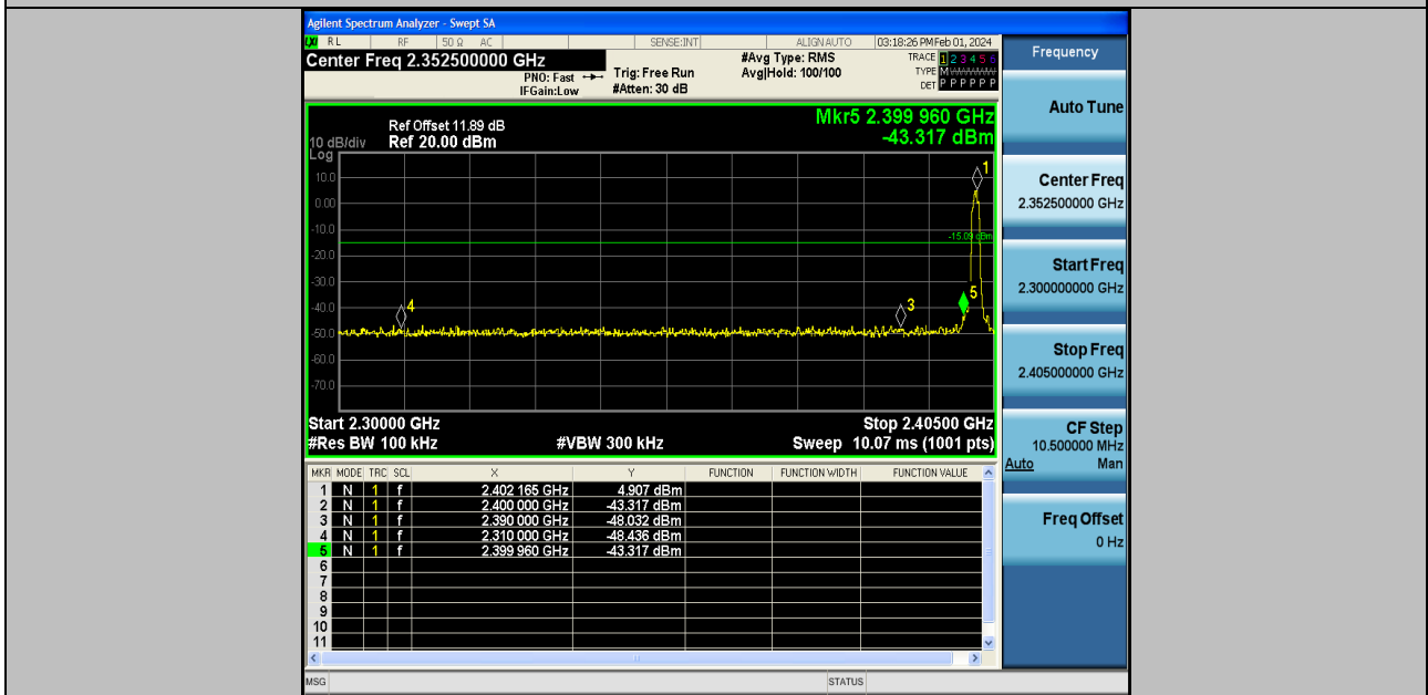
3DH5-Ant2-2402-PASS
