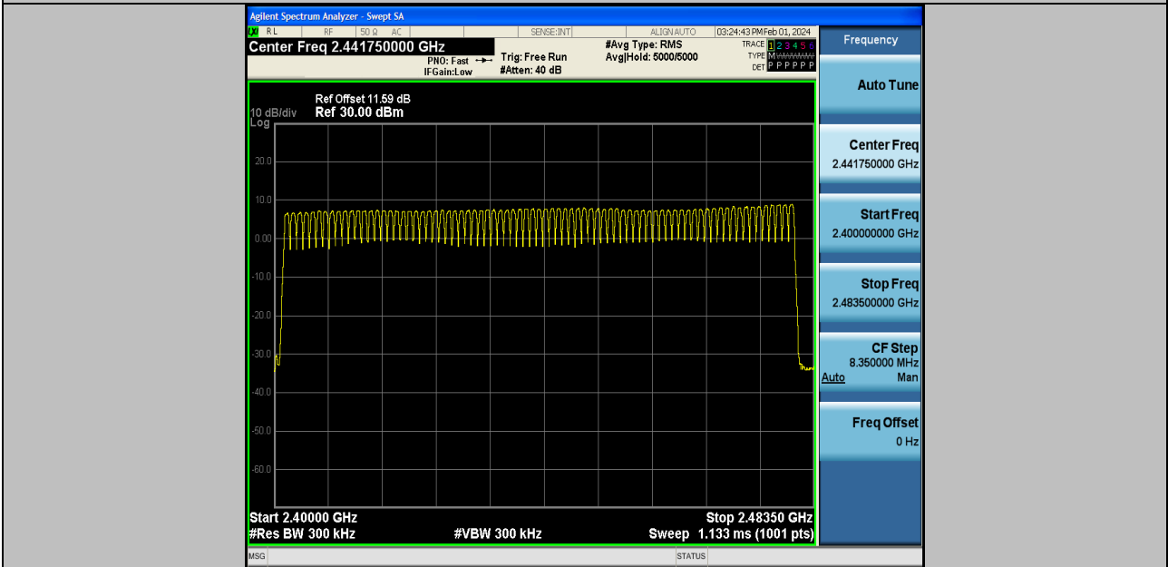
DH5-Ant2-Hop-PASS
