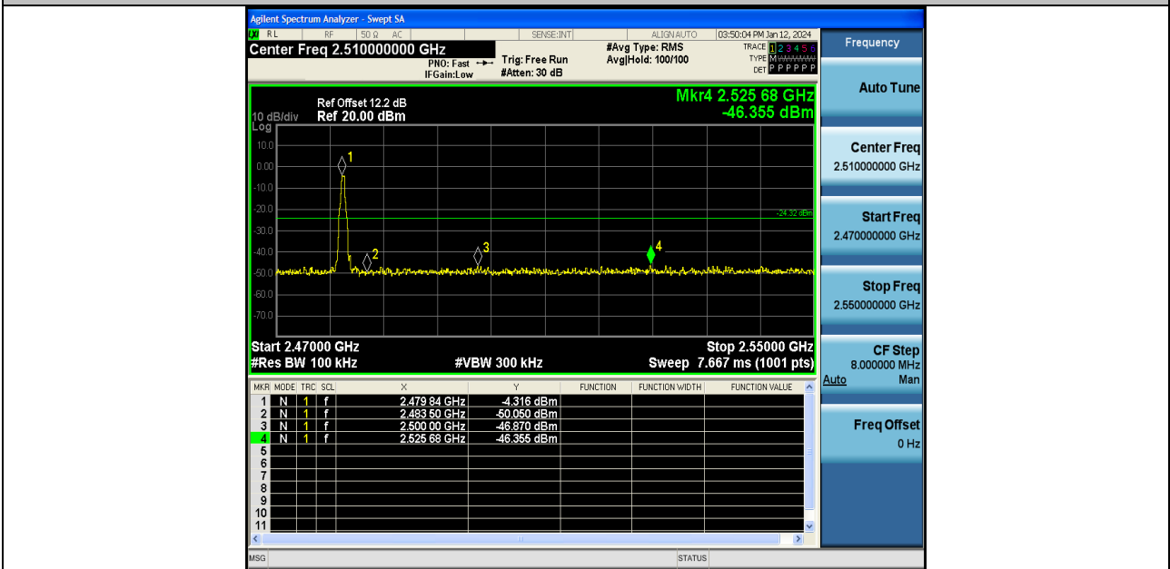
DH5-Ant1-2480-PASS
