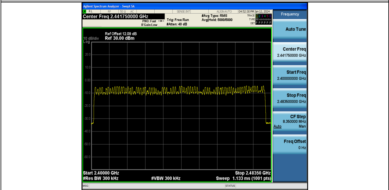
2DH5-Ant1-Hop-PASS
