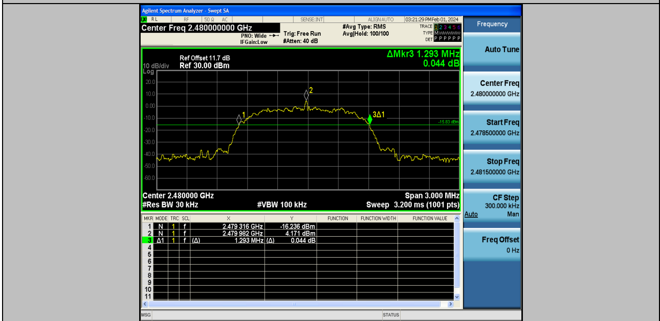
3DH5-Ant2-2480
