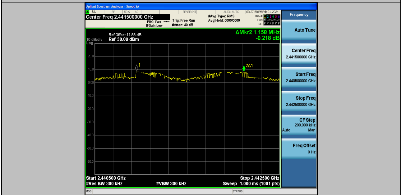
2DH5-Ant2-Hop-PASS
