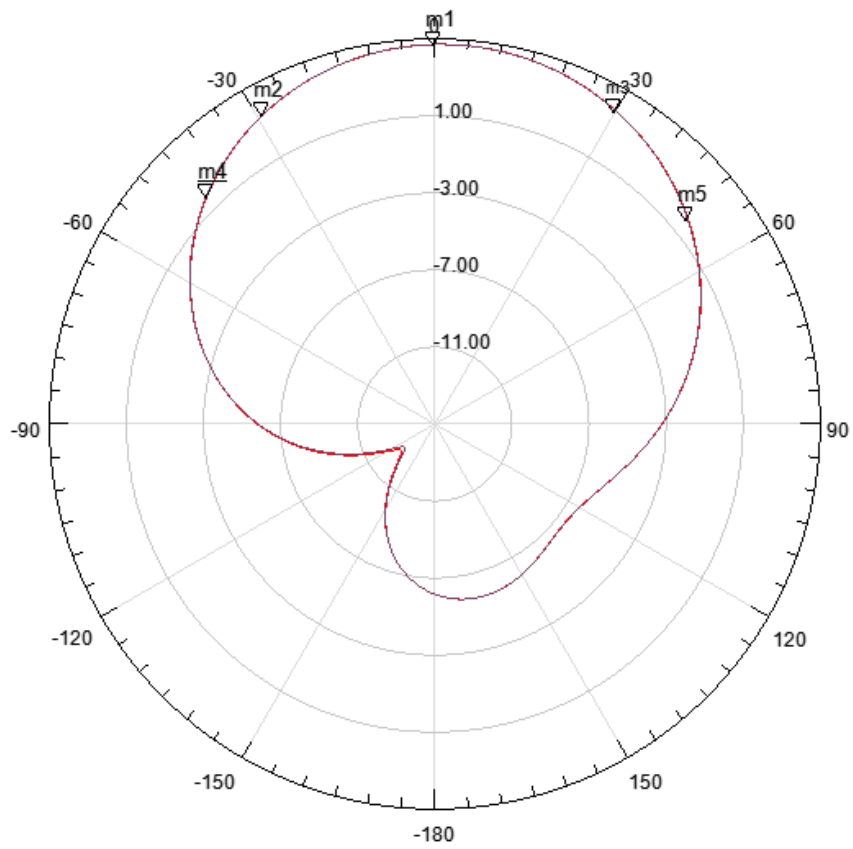
Radiation Pattern 1
