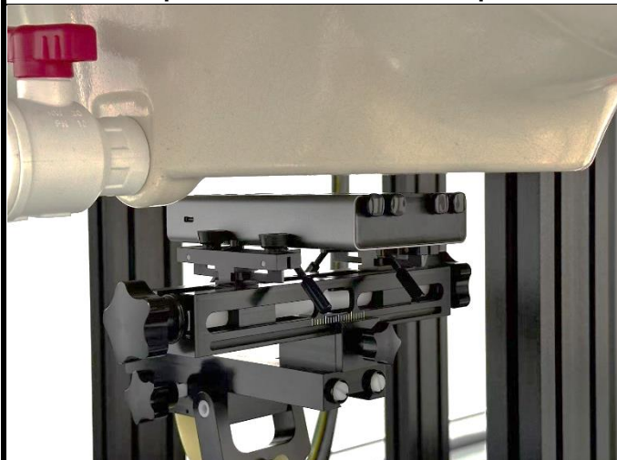
Rear Face of EUT + Probe with 1cm Gap
