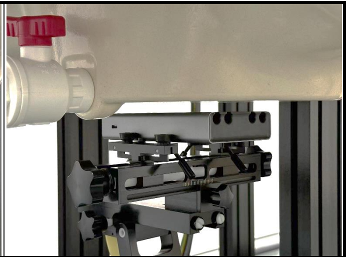
Rear Face of EUT with 1 cm Gap
