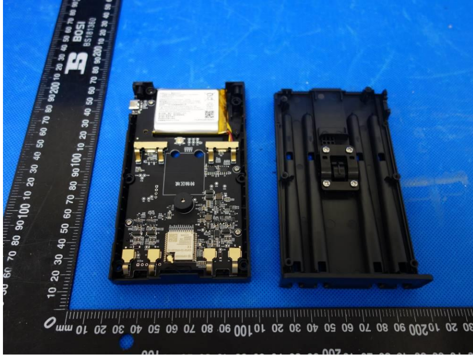
Figure 5: Internal view (Device Base)
