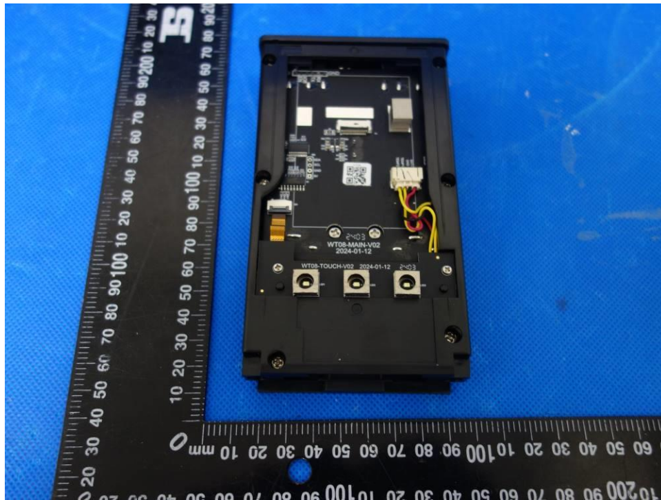
Figure 4: Internal view (Device Base)
