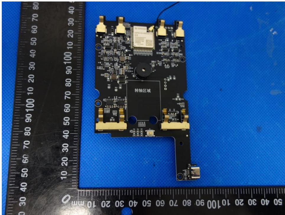
Figure 10: Main PCB (Device Base)
