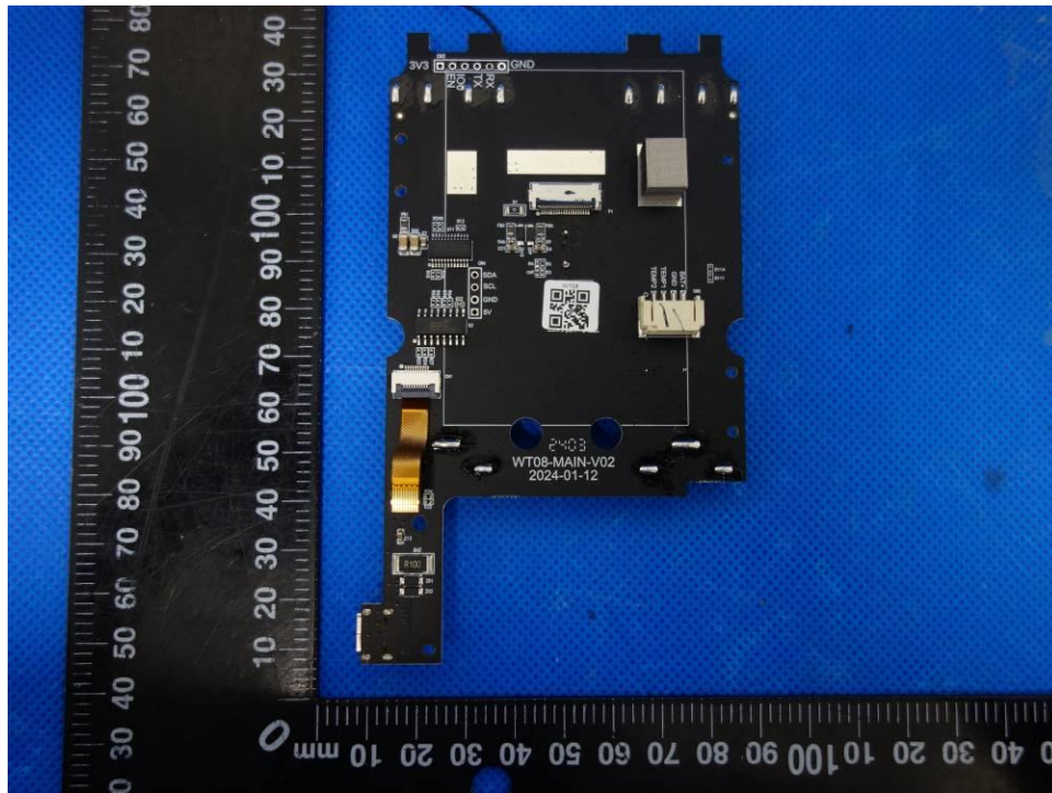
Figure 11: Main PCB (Device Base)
