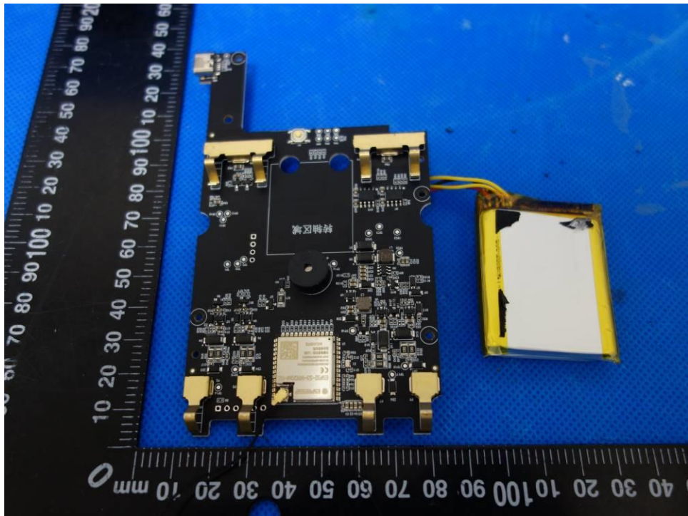
Figure 8: Internal view (Device Base)
