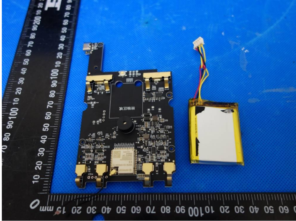
Figure 9: Internal view (Device Base)
