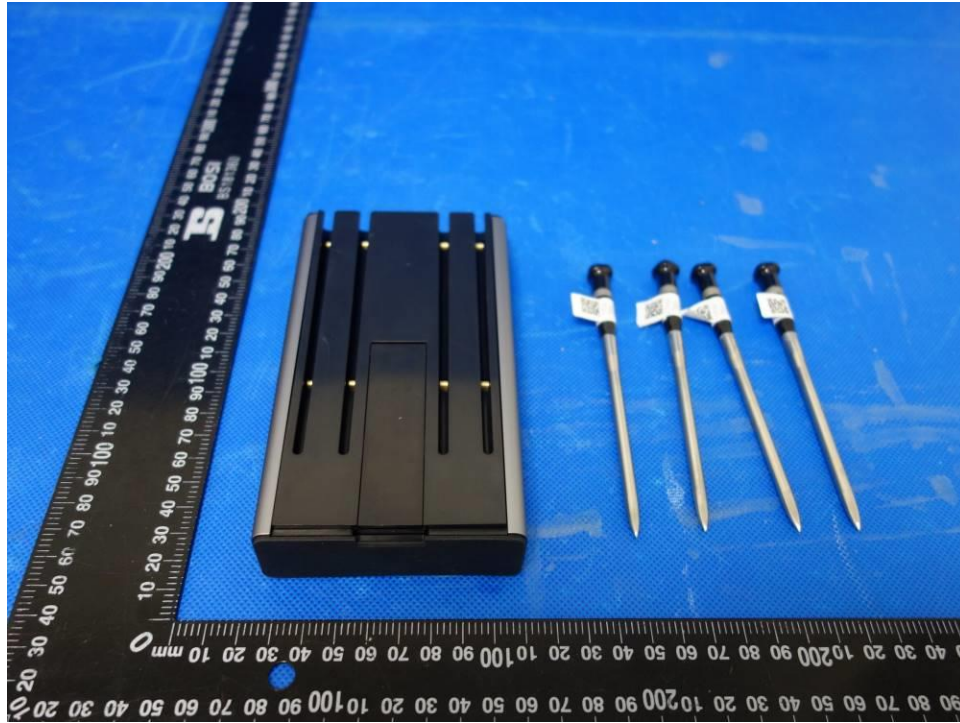
Figure 7: Overview (Device Base and Probe)
