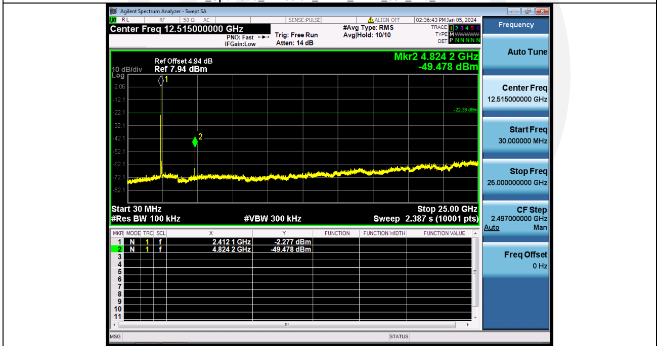
2_Spurious_Emission_NVNT_ANT1_802_11b_2412
