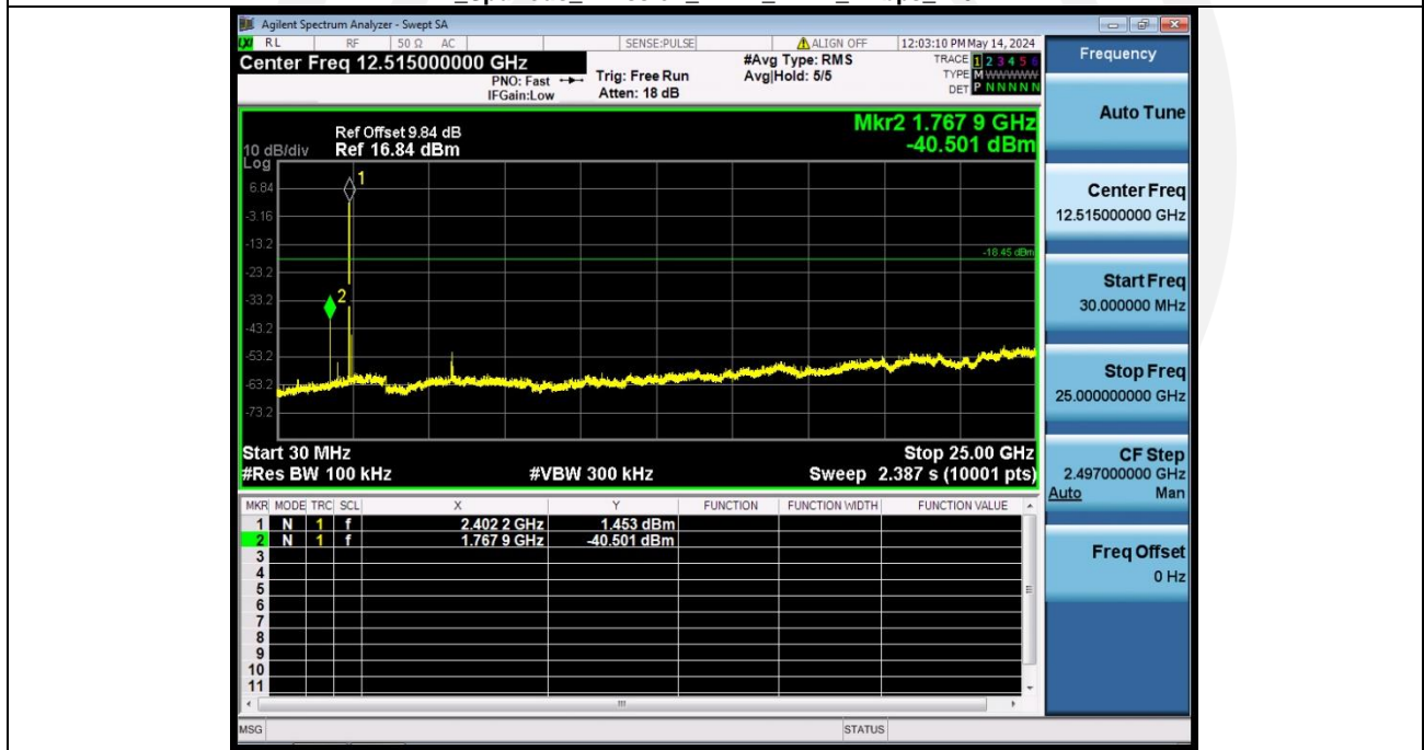
2_Spurious_Emission_NVNT_ANT1_1Mbps_2402
