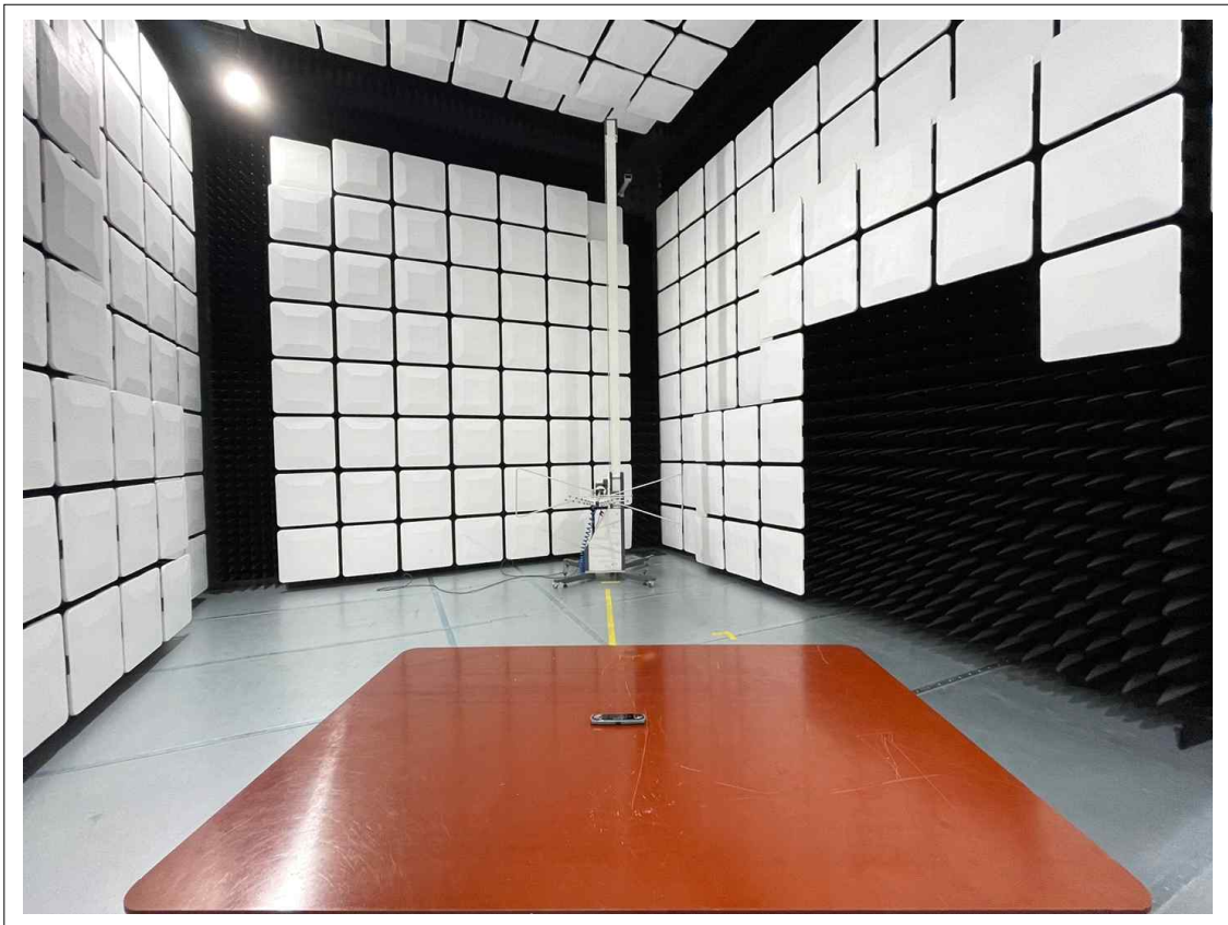
Radiated Emission Test Setup Below 1GHz_H
