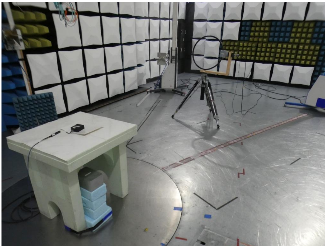
Photo 1: Test setup for radiated measurements, under 30 MHz
