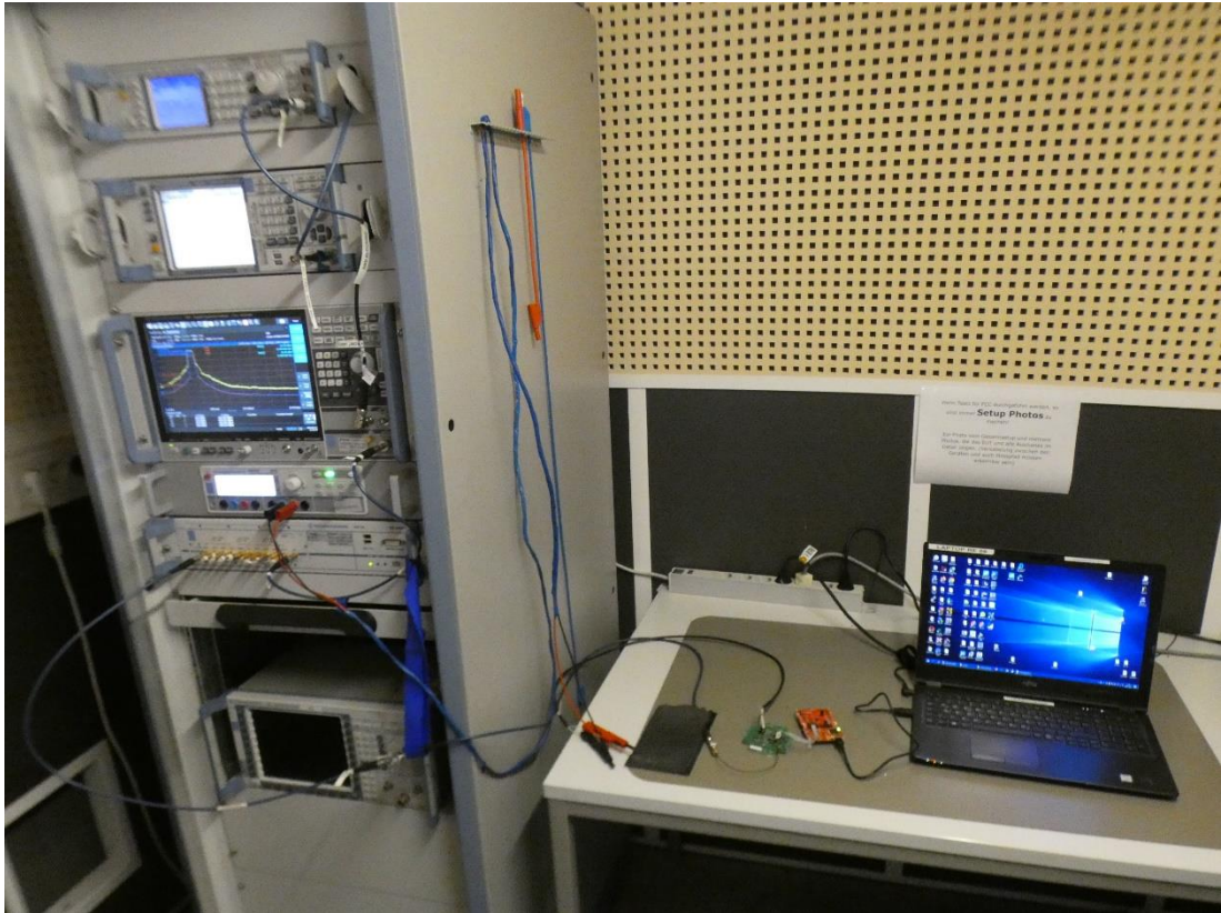
Photo 5: Test setup for conducted measurements
