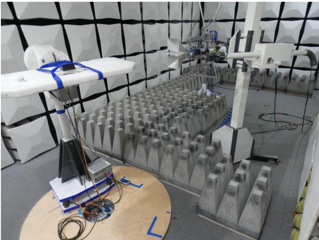
Photo 4: Test setup for radiated measurements, Band Edge Compliance
