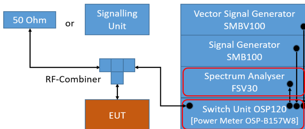
TS8997; Output Power
