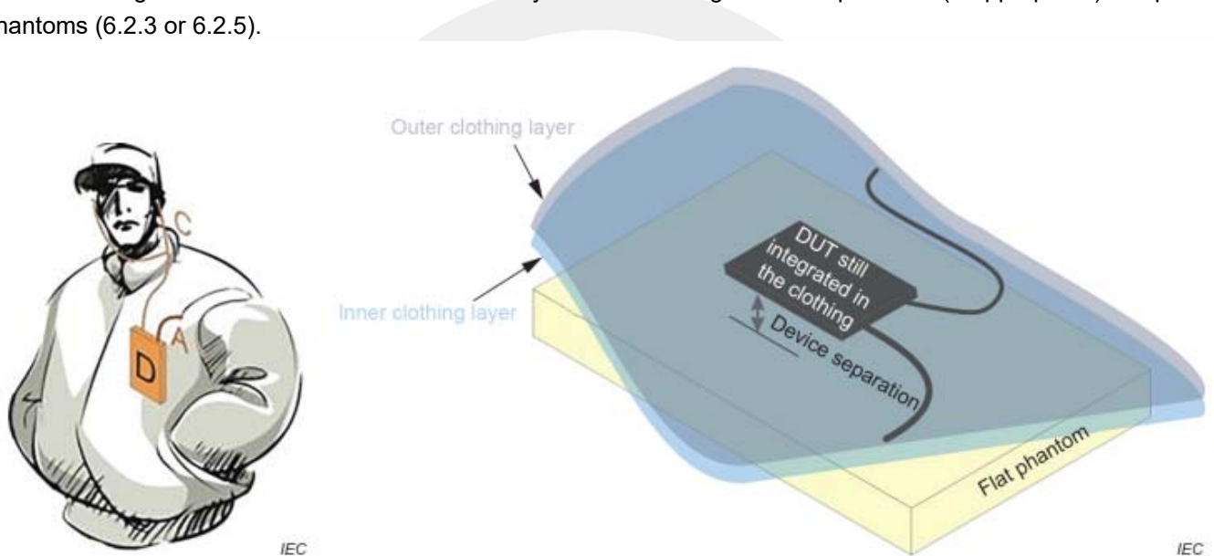
Fig-4.1 Test position for clothing-integrated wireless communication devices
