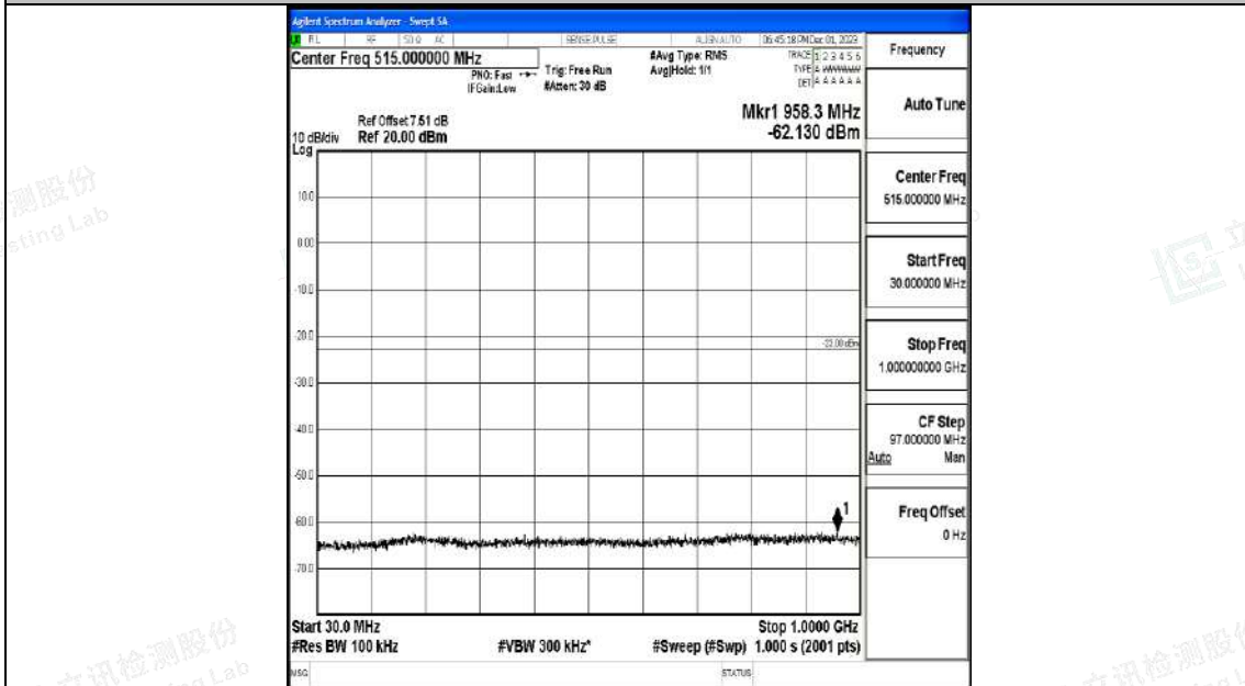
Band2_3MHz_16QAM_18615_1RB#0_30~1000_30~1000
