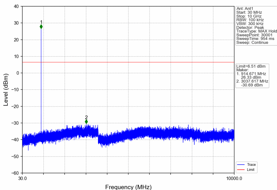
150kbps_MCH_914.8MHz_Ant1_NTNV
