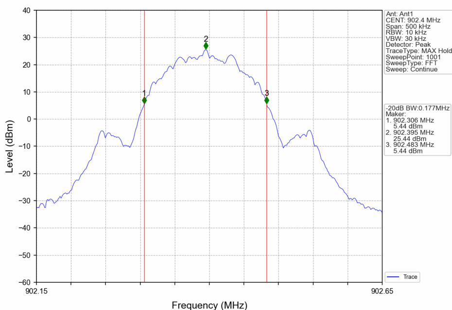
150kbpd_LCH_902.4MHz_Ant1_NTNV
