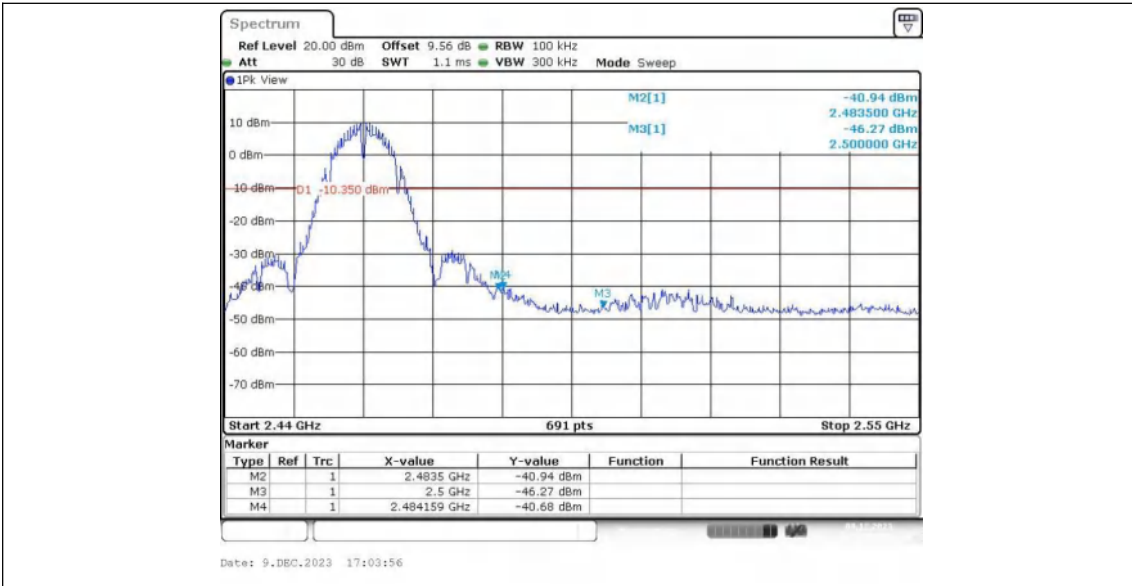
11B_Ant2_High_2462
