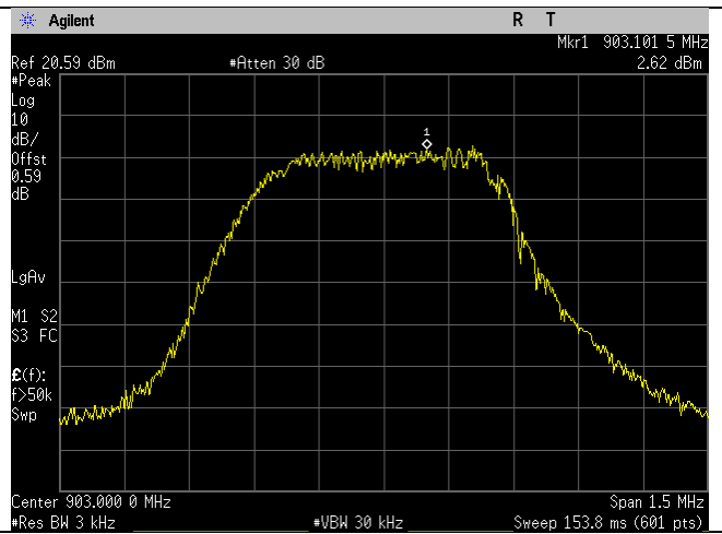
Low Ch_903MHz_Spectral_Density
