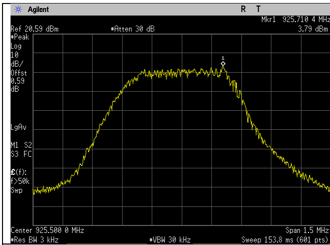
High Ch_925.5MHz_Spectral_Density
