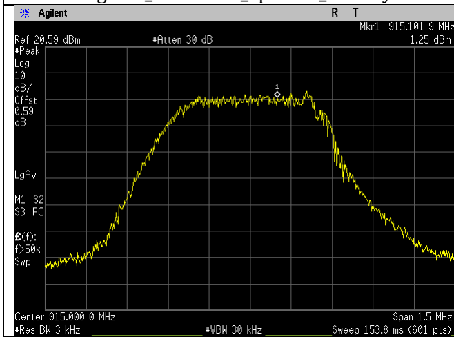
Mid Ch_915MHz_Spectral_Density
