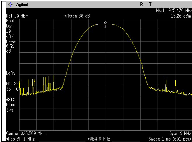
High Ch_925.5MHz_Ouput_Power
