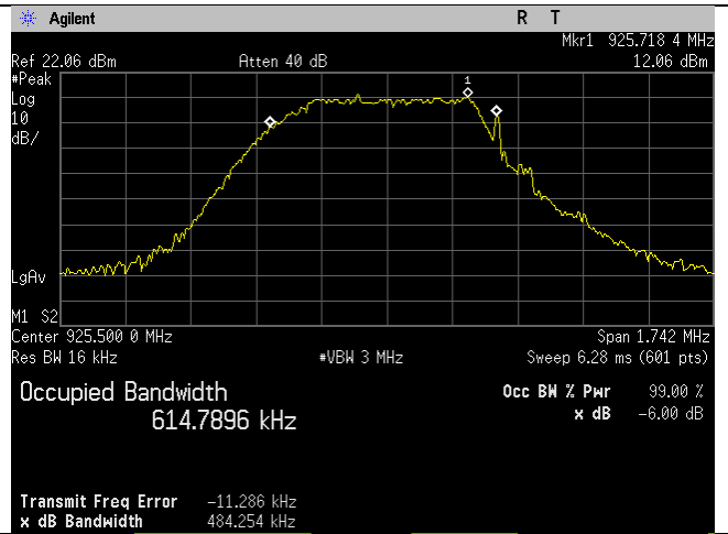
High Ch_925.5MHz_1MBit_Occupied Bandwidth_99 percent
