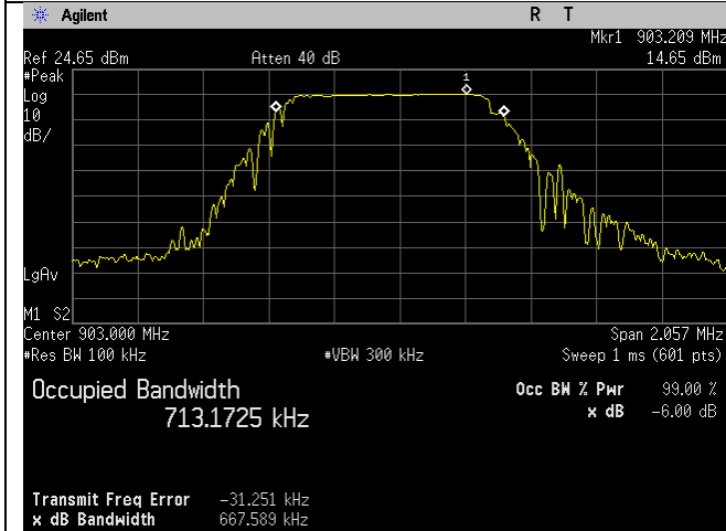
Low Ch_903MHz_1MBit_Occupied Bandwidth_-6dB
