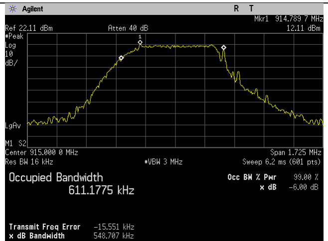
Mid Ch_915MHz_1MBit_Occupied Bandwidth_99 percent
