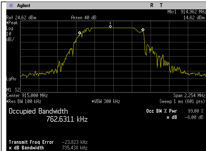
Mid Ch_915MHz_1MBit_Occupied Bandwidth_-6dB
