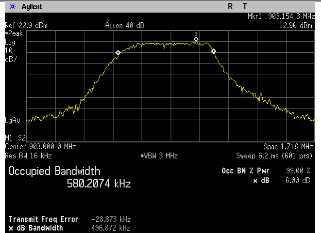
Low Ch_903MHz_1MBit_Occupied Bandwidth_99 percent
