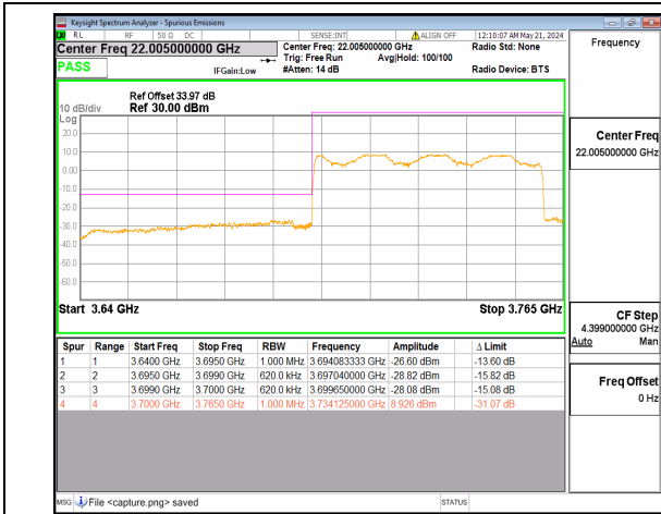
n77(3700-3980MHz) 60M DFT-s-OFDM QPSK Outer_Full Low
