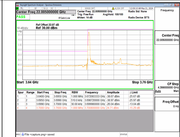
n77(3700-3980MHz) 60M DFT-s-OFDM BPSK Edge_1RB_Left Low
