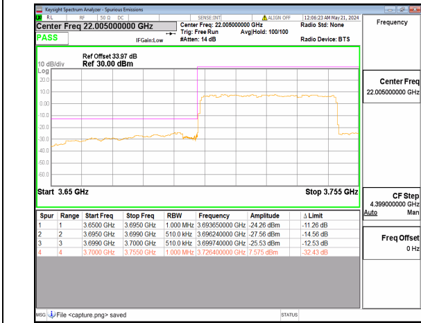
n77(3700-3980MHz) 50M DFT-s-OFDM QPSK Outer_Full Low
