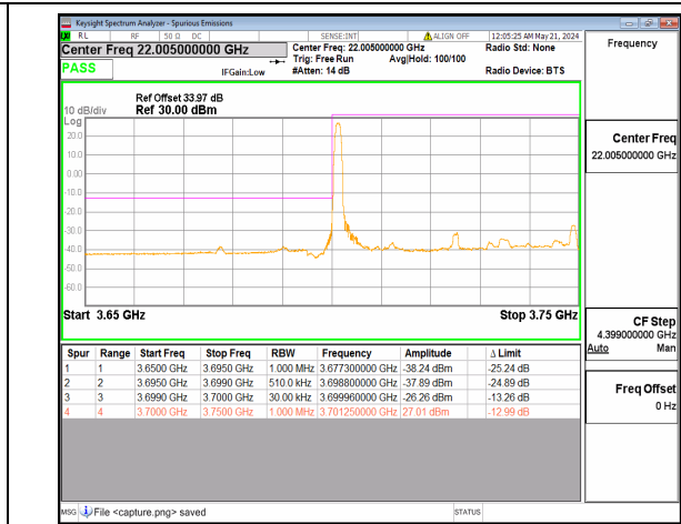
n77(3700-3980MHz) 50M DFT-s-OFDM BPSK Edge_1RB_Left Low
