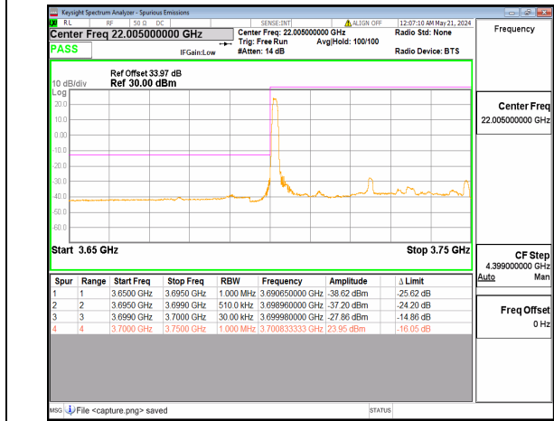
n77(3700-3980MHz) 50M DFT-s-OFDM QPSK Edge_1RB_Left Low
