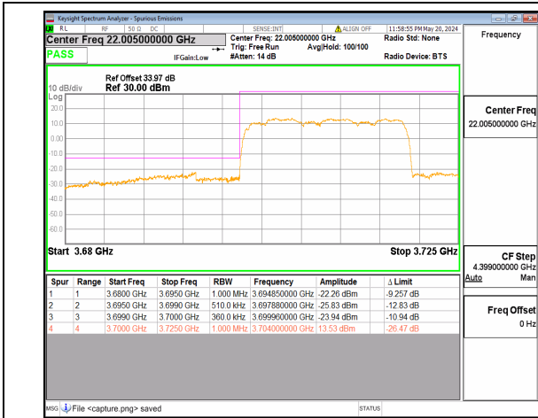
n77(3700-3980MHz) 20M DFT-s-OFDM QPSK Outer_Full Low
