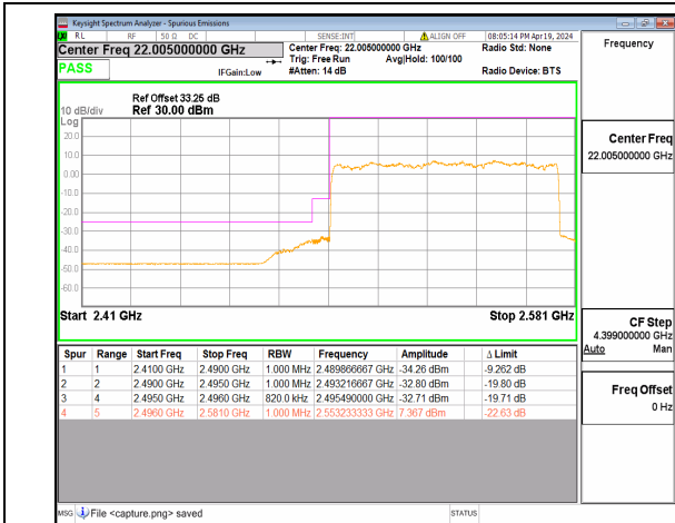
n41 80M DFT-s-OFDM QPSK Outer_Full Low
