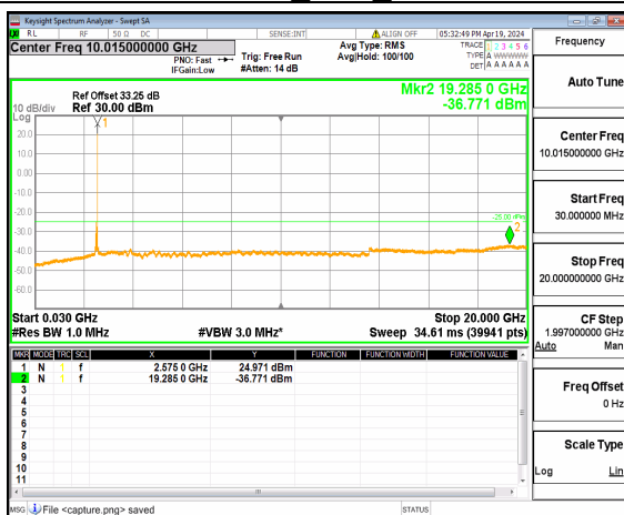
n41 (30MHz-20GHz) 80M DFT-s-OFDM BPSK Inner_1RB_Right Low
