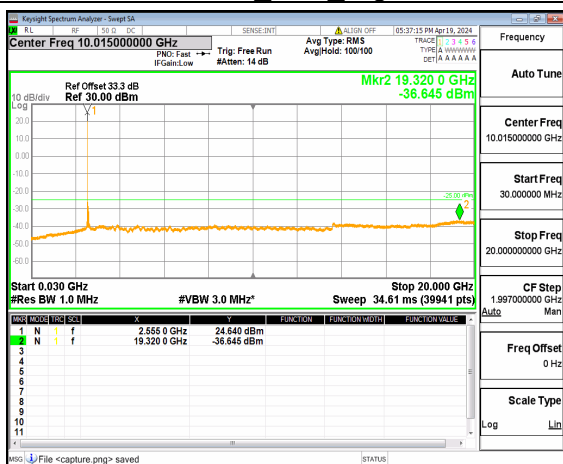
n41 (30MHz-20GHz) 80M DFT-s-OFDM BPSK Inner_1RB_Left Mid
