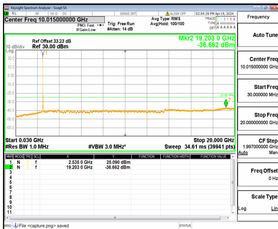
n41 (30MHz-20GHz) 40M DFT-s-OFDM BPSK Inner_1RB_Right Low
