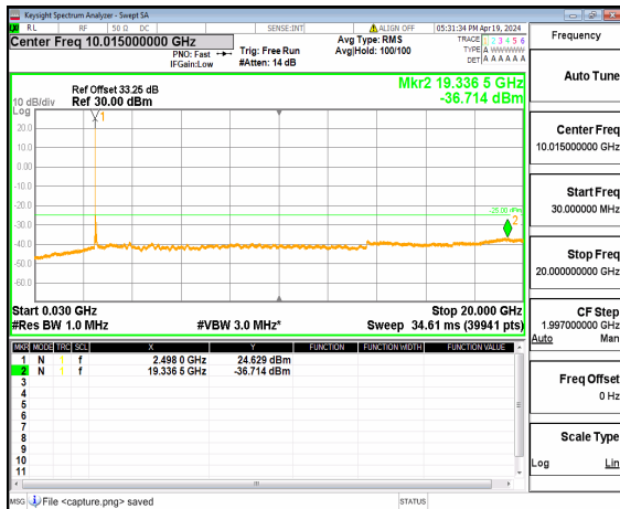
n41 (30MHz-20GHz) 80M DFT-s-OFDM BPSK Inner_1RB_Left Low
