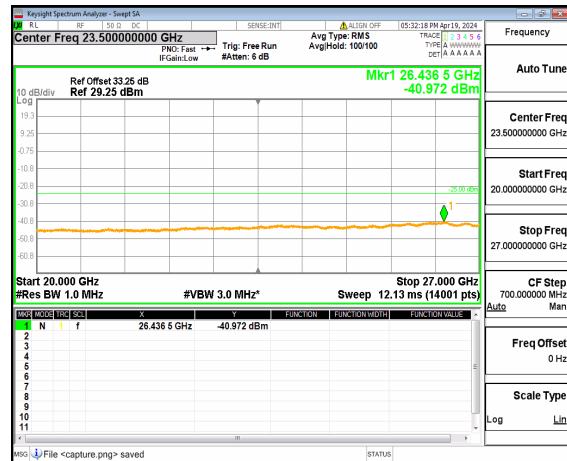
n41 (20GHz-27GHz) 80M DFT-s-OFDM BPSK Inner_1RB_Left Low
