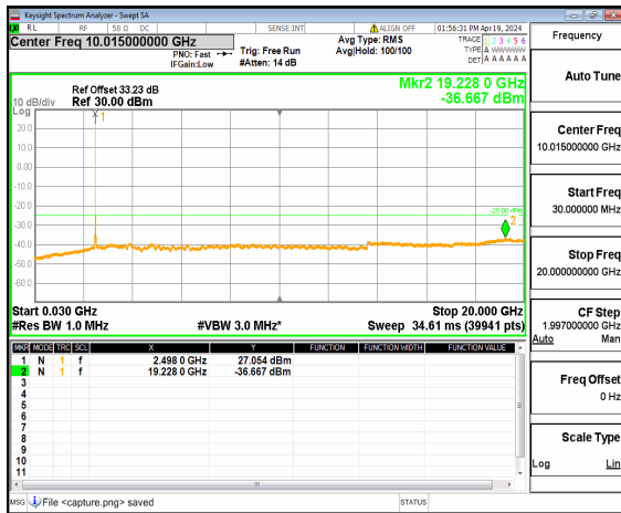
n41 (30MHz-20GHz) 40M DFT-s-OFDM BPSK Inner_1RB_Left Low
