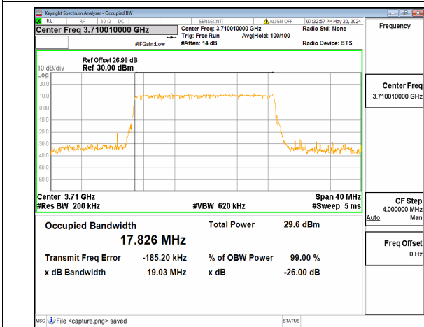
n77(3700-3980MHz) 20M DFT-s-OFDM 256QAM Outer_Full Low
