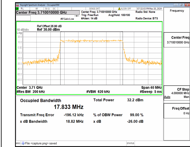
n77(3700-3980MHz) 20M DFT-s-OFDM 16QAM Outer_Full Low
