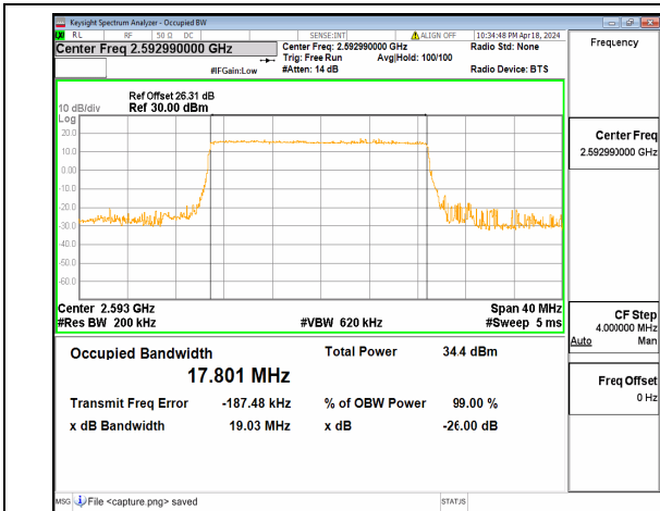
n41 20M DFT-s-OFDM BPSK Outer_Full Mid
