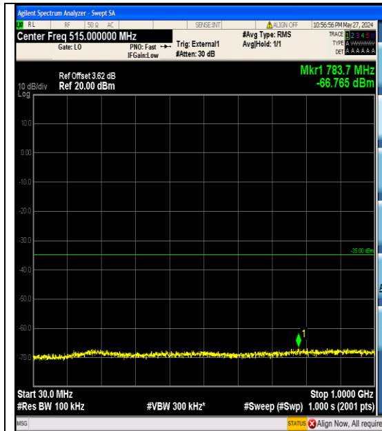
Band41_20MHz_16QAM_40590_100RB#0_30~1000_30~1000
