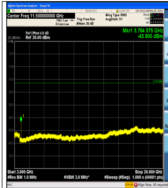
Band25_3MHz_16QAM_26365_15RB#0_3000~ 20000_3000~20000
