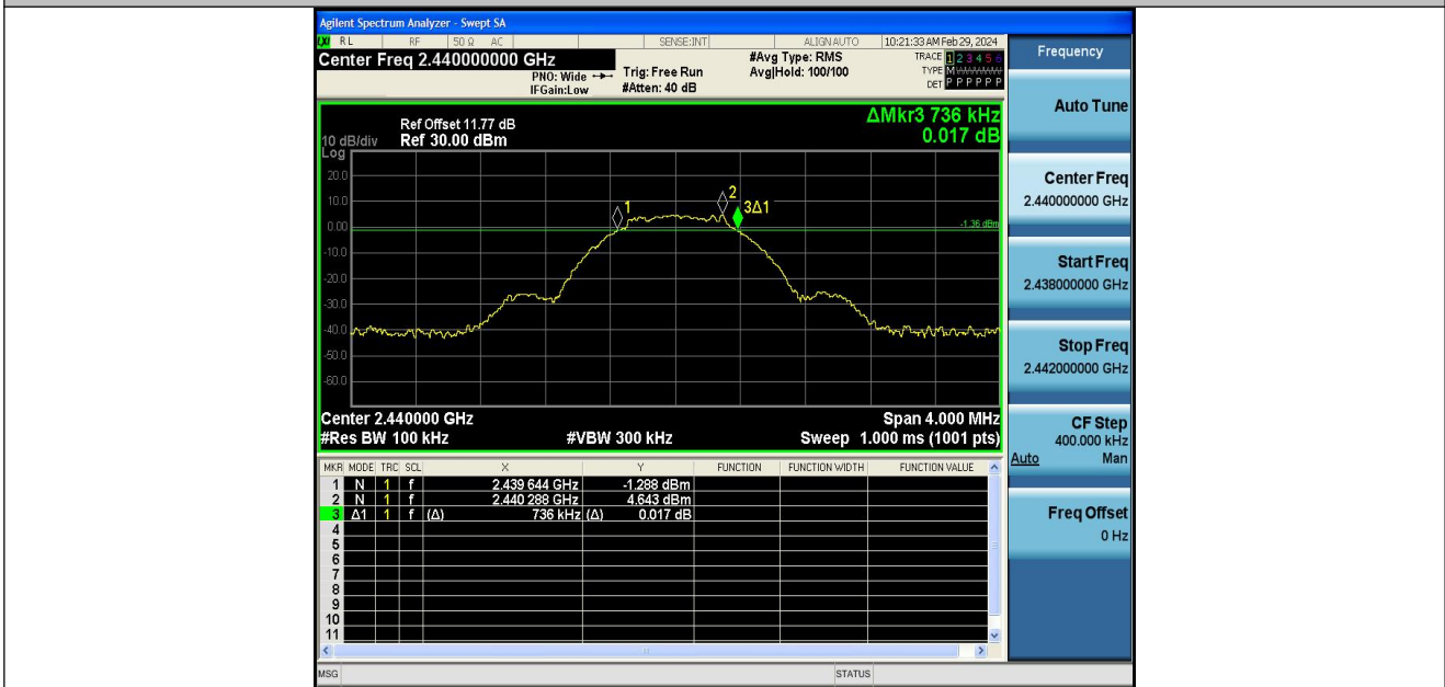
BLE_1M-Ant1-2440-PASS
